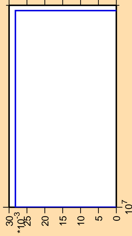
\Delta\sigma/\sigma vs. E for ^{213}\text{Pb} (mt 11)
