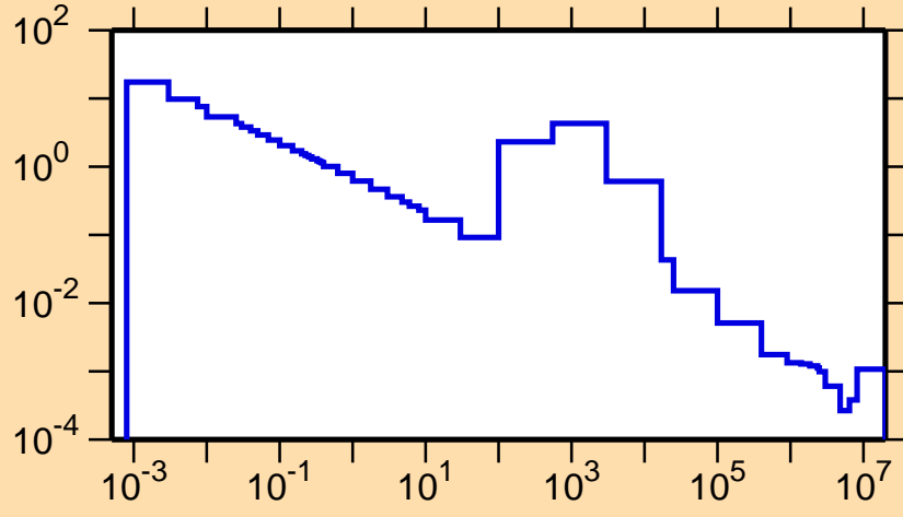
\sigma vs. E for ^{213}\text{Pb}(n,\gamma)
