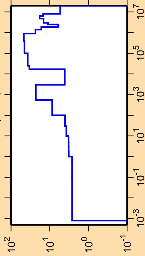
\Delta\sigma/\sigma vs. E for ^{213}\text{Pb}(n,\text{el.})
