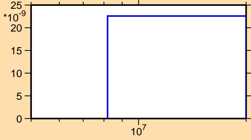
\sigma vs. E for ^{213}\text{Pb}(n,2n\alpha)
