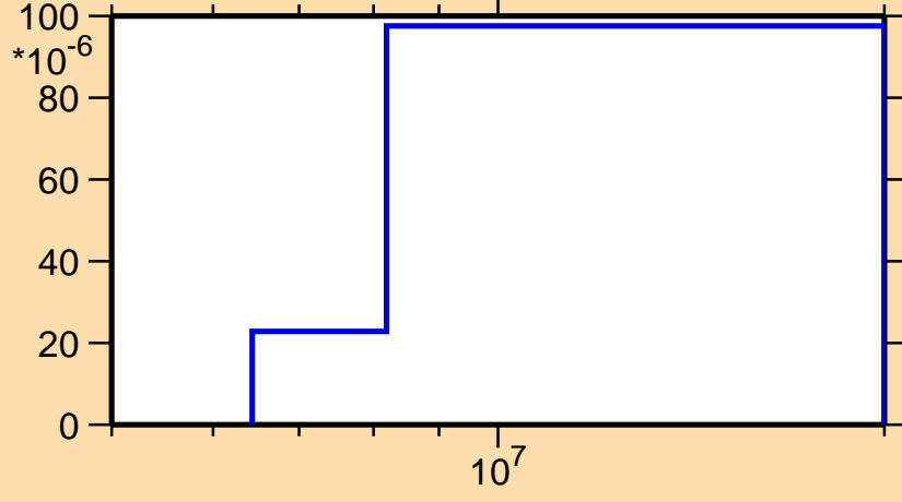
\sigma vs. E for ^{213}\text{Pb}(n,n\alpha)
