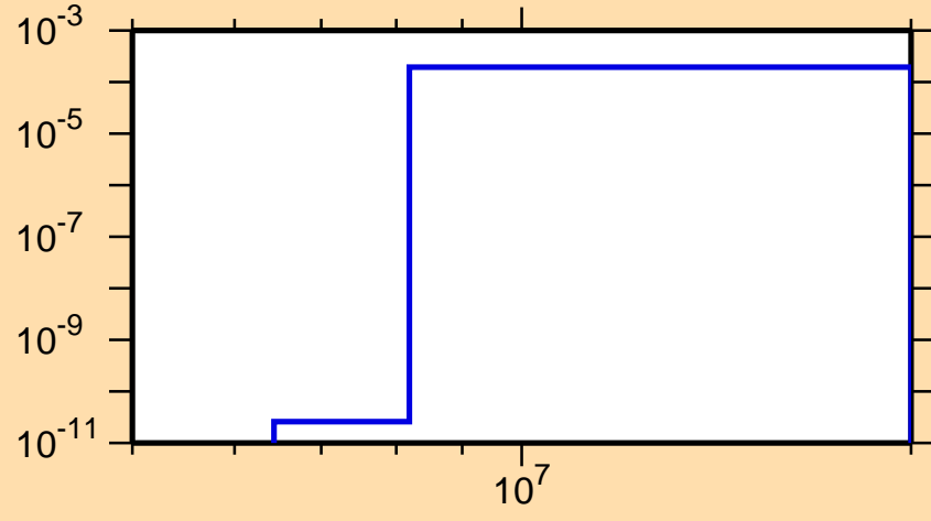
\sigma vs. E for ^{213}\text{Pb}(n,p)
