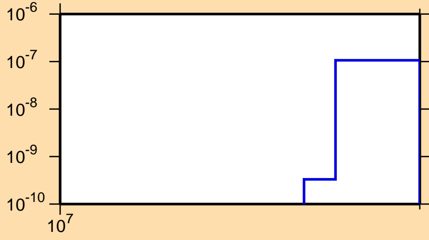
\sigma vs. E for ^{215}\text{Pb}(n,2np)
