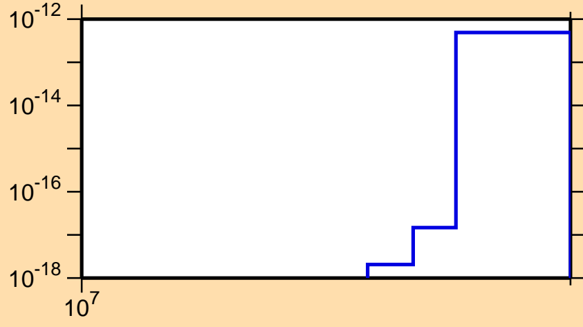
\sigma vs. E for ^{215}\text{Pb}(\text{mt } 11)
