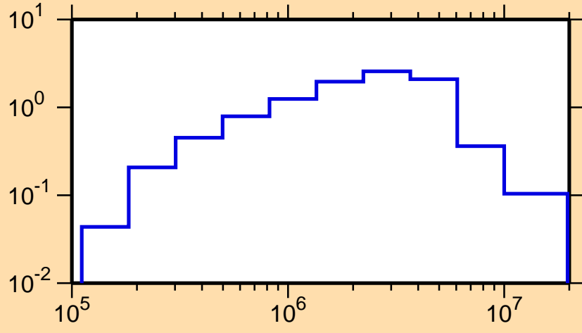
\sigma vs. E for ^{215}\text{Pb}(n,\text{inel.})
