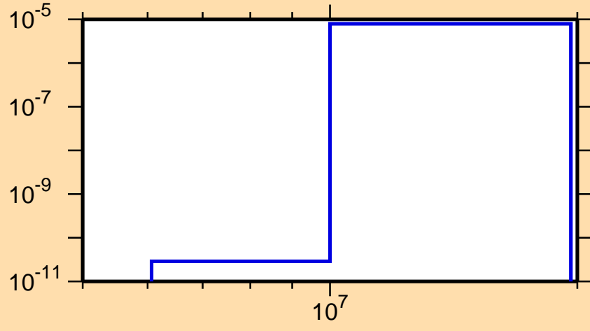
\sigma vs. E for ^{215}\text{Pb}(n,n\alpha)
