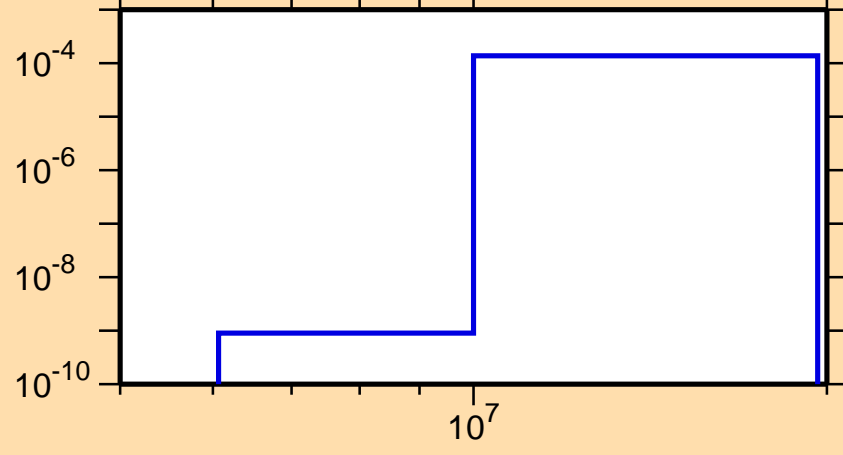
\sigma vs. E for ^{215}\text{Pb}(n,p)
