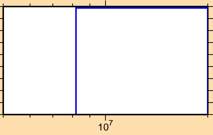
\sigma vs. E for ^{215}\text{Pb}(n,nt)
