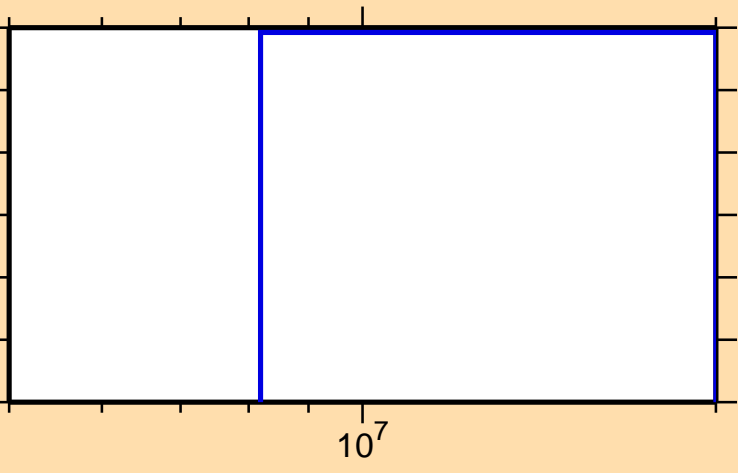
\sigma vs. E for ^{215}\text{Pb}(n,\text{nd})
