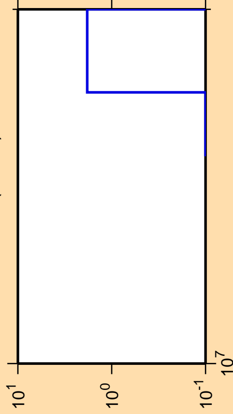
\Delta\sigma/\sigma vs. E for ^{217}\text{Pb} (mt 11)
