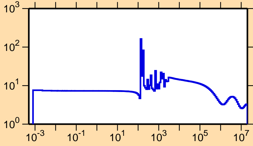
\sigma vs. E for ^{217}\text{Pb}(n,\text{el.})
