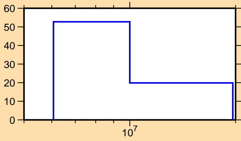
\Delta\sigma/\sigma vs. E for ^{217}\text{Pb}(n,\text{el.})
