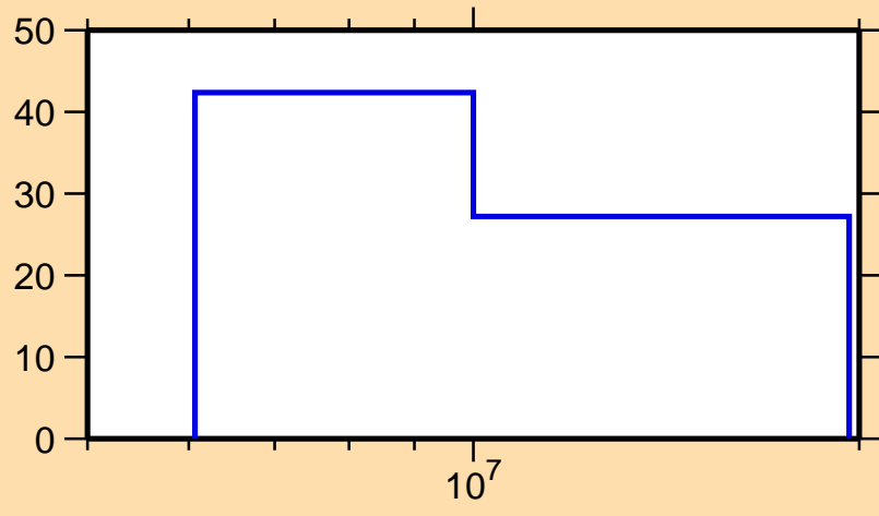
\Delta\sigma/\sigma vs. E for ^{217}\text{Pb}(n,\text{tot.})
