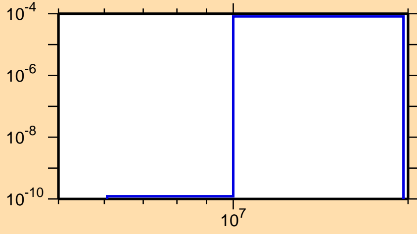
\sigma vs. E for ^{217}\text{Pb}(n,p)
