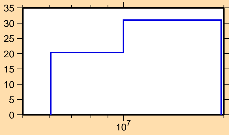
\Delta\sigma/\sigma vs. E for ^{217}\text{Pb}(n,2n)
