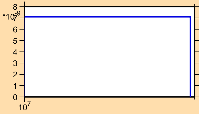
\sigma vs. E for ^{217}\text{Pb}(n,\text{nd})
