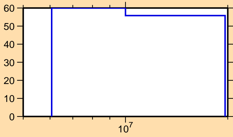
\Delta\sigma/\sigma vs. E for ^{217}\text{Pb}(n,n_1)
