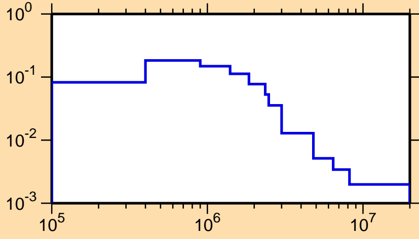
\sigma vs. E for ^{217}\text{Pb}(n,n_1)
