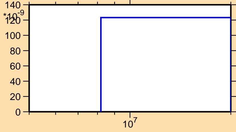
\sigma vs. E for ^{217}\text{Pb}(n,nt)
