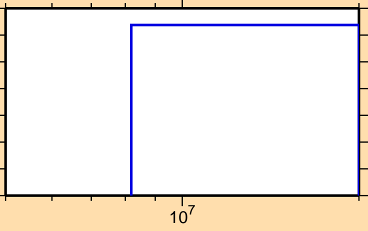
\sigma vs. E for ^{217}\text{Pb}(n,t)
