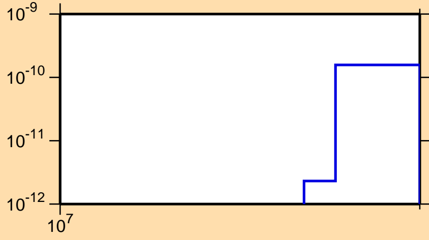
\sigma vs. E for ^{218}\text{Pb}(n,3n\alpha)
