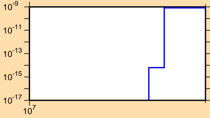
\sigma vs. E for ^{218}\text{Pb}(n,2np)
