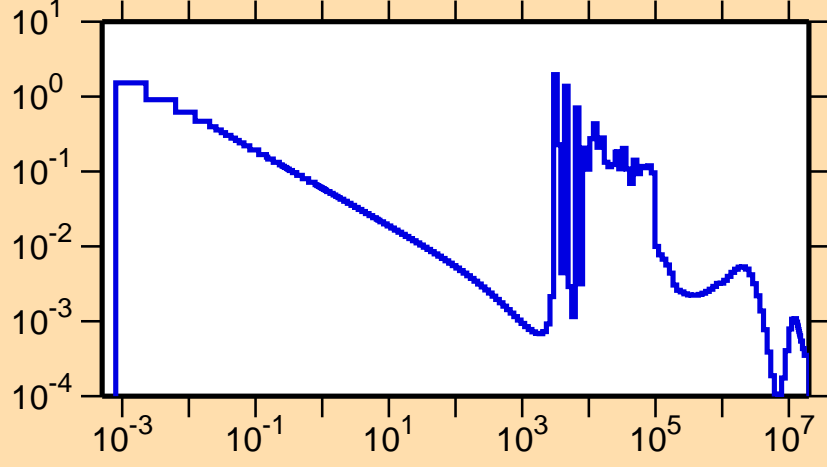
\sigma vs. E for ^{218}\text{Pb}(n,\gamma)
