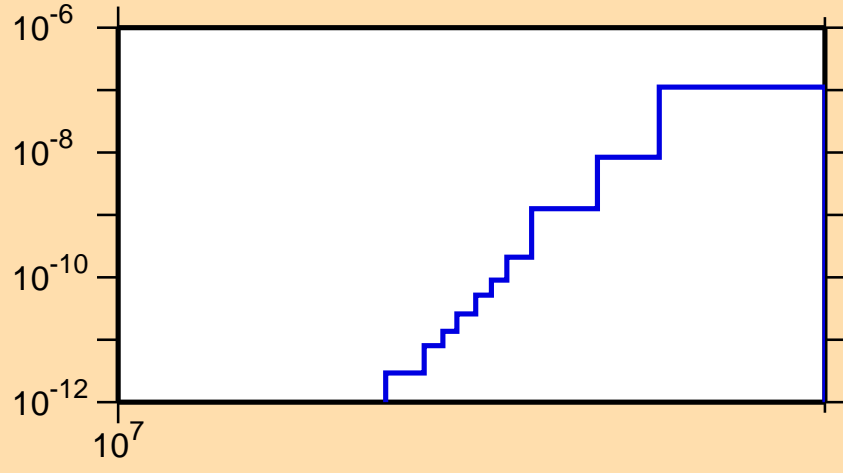
\sigma vs. E for ^{218}\text{Pb}(n,2n\alpha)
