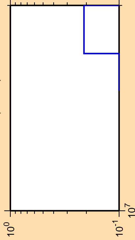
\Delta\sigma/\sigma vs. E for ^{218}\text{Pb} (mt 11)
