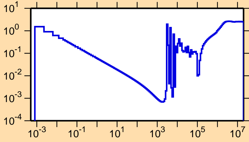
\sigma vs. E for ^{218}\text{Pb}(n,\text{nonel.})
