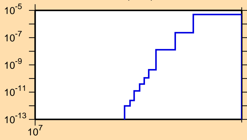
\sigma vs. E for ^{218}\text{Pb}(n,nt)
