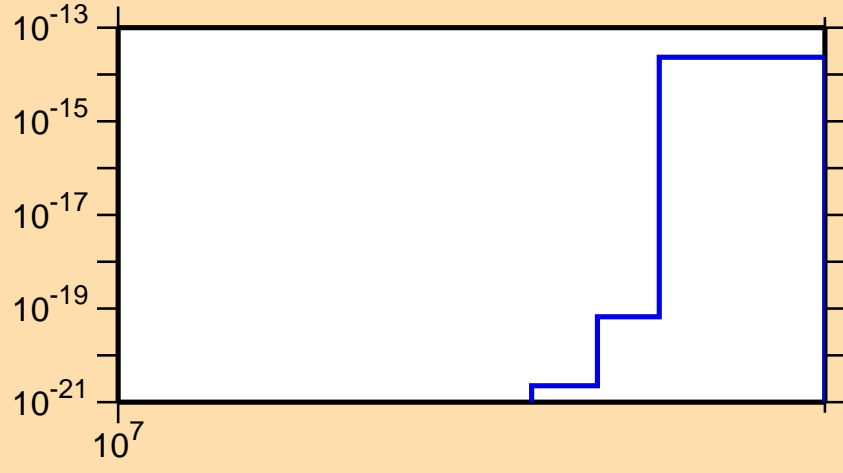
\sigma vs. E for ^{218}\text{Pb} (mt 11)
