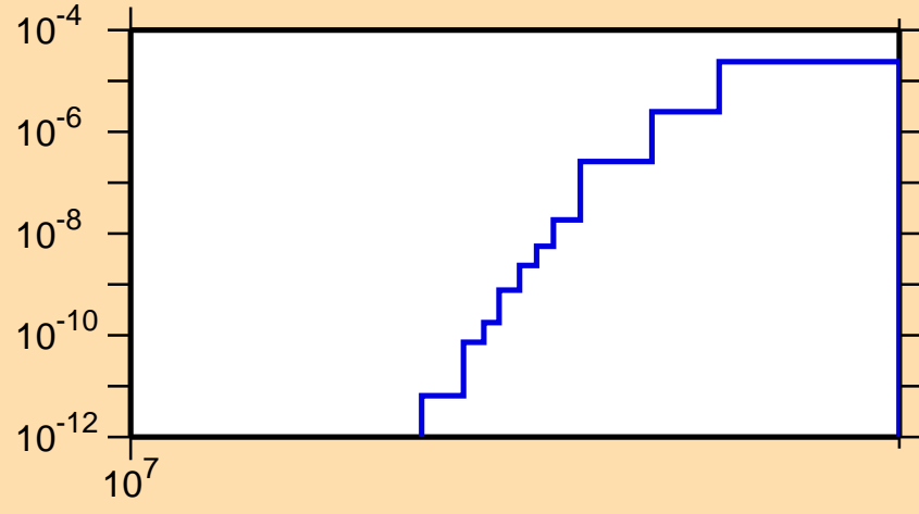
\sigma vs. E for ^{218}\text{Pb}(n,np)
