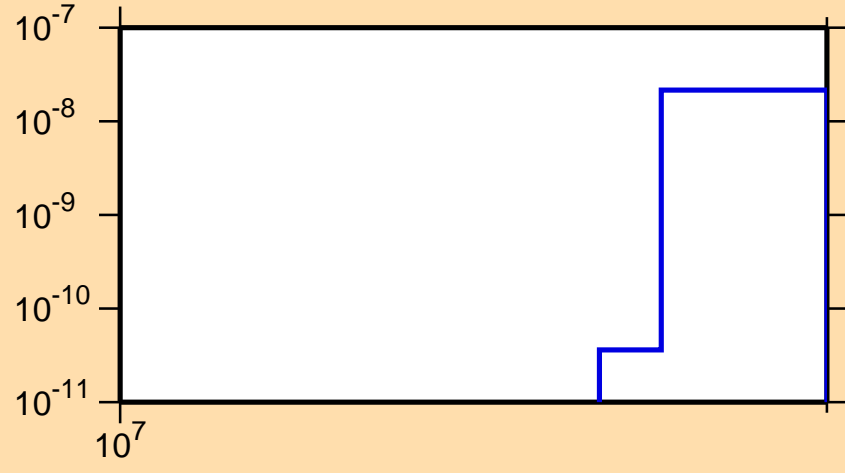
\sigma vs. E for ^{218}\text{Pb}(n,\text{nd})
