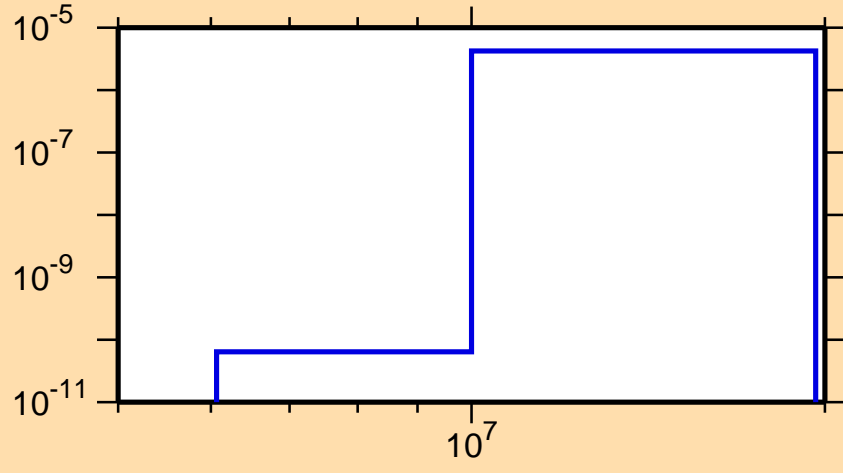
\sigma vs. E for ^{218}\text{Pb}(n,\alpha)
