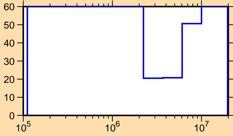
\Delta\sigma/\sigma vs. E for ^{218}\text{Pb}(n, tot.)
