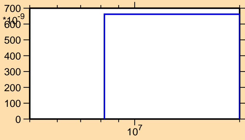
\sigma vs. E for ^{218}\text{Pb}(n,d)
