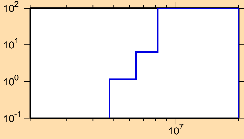
\Delta\sigma/\sigma vs. E for ^{218}\text{Pb}(n,2n)
