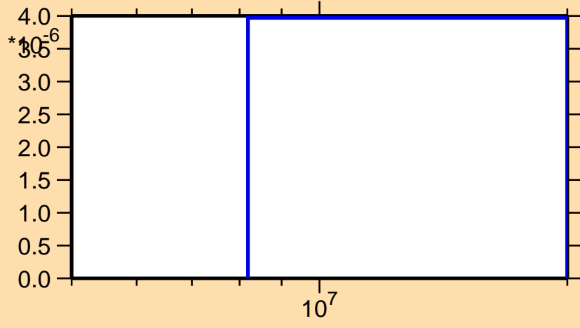
\sigma vs. E for ^{218}\text{Pb}(n,t)
