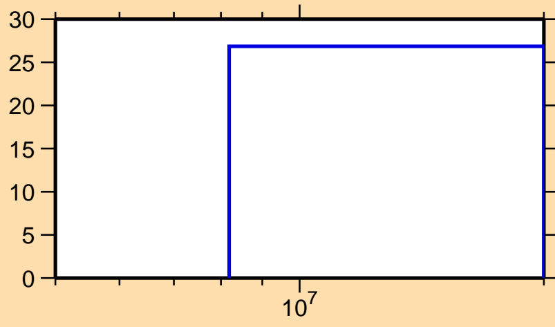
\Delta\sigma/\sigma vs. E for ^{218}\text{Pb}(n,n\text{cont.})
