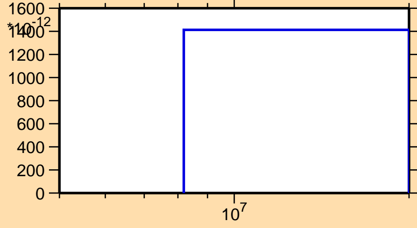
\sigma vs. E for ^{218}\text{Pb}(n,2n\alpha)
