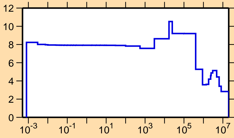
\sigma vs. E for ^{218}\text{Pb}(n,\text{el.})
