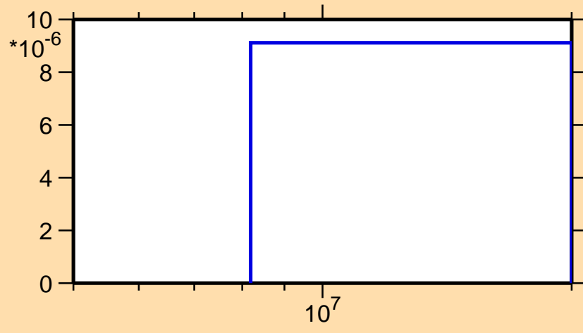
\sigma vs. E for ^{218}\text{Pb}(n,p)
