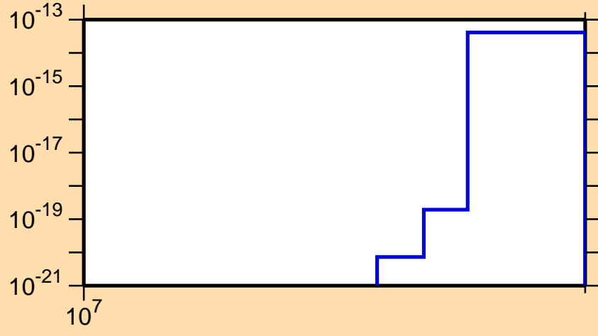
\sigma vs. E for ^{219}\text{Pb}(\text{mt } 11)
