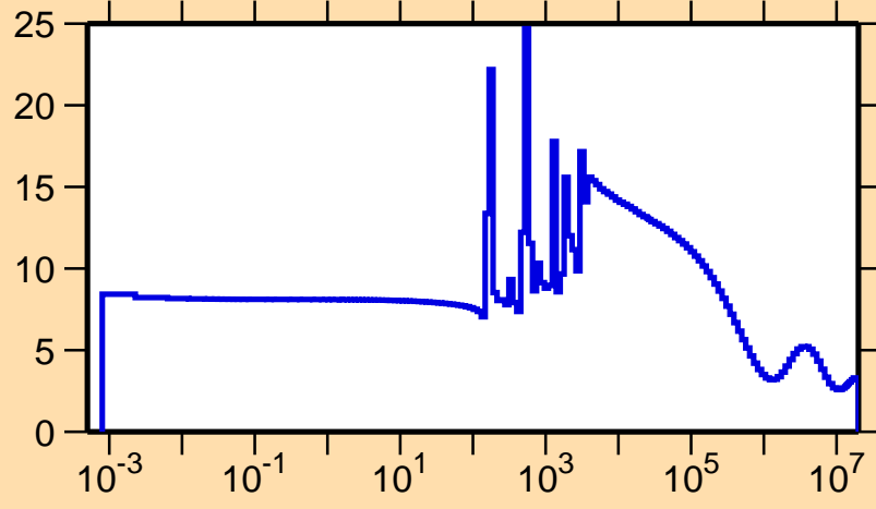
\sigma vs. E for ^{219}\text{Pb}(n,\text{el.})
