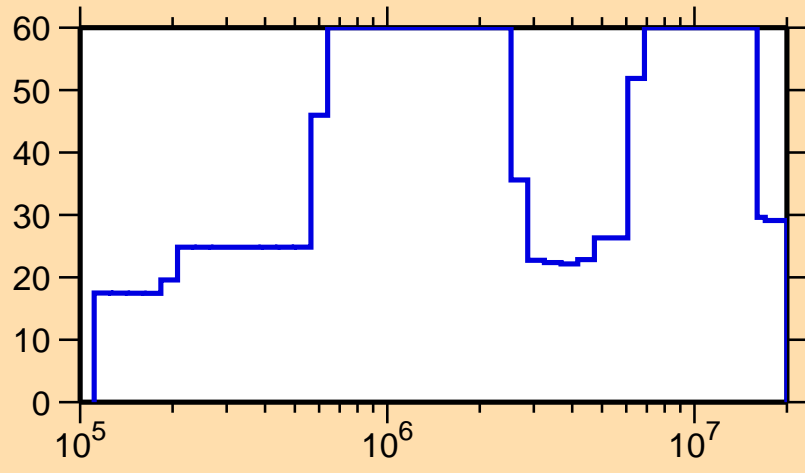
\Delta\sigma/\sigma vs. E for ^{219}\text{Pb}(n, el.)
