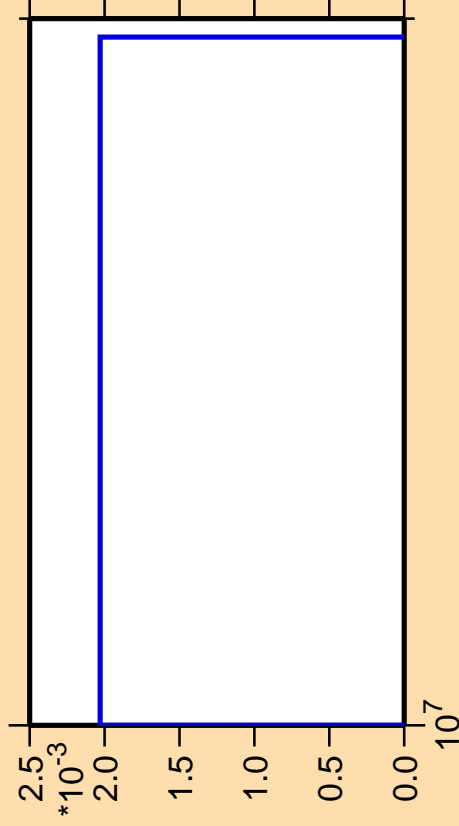
\Delta\sigma/\sigma vs. E for ^{219}\text{Pb} (mt 11)
