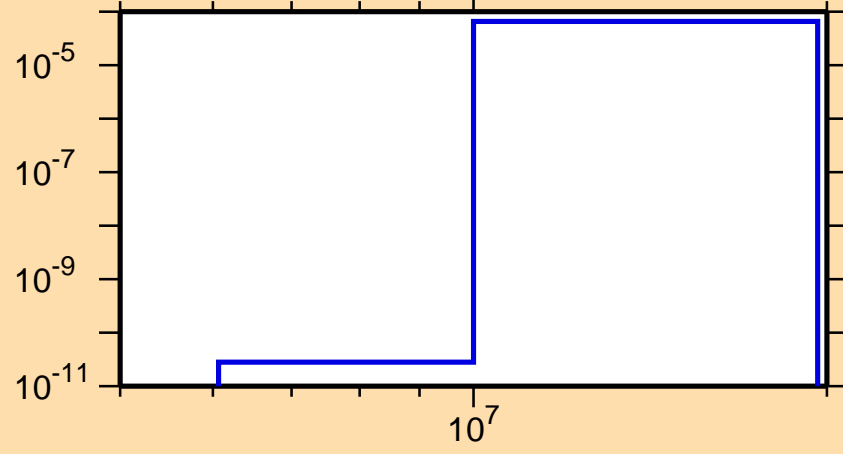
\sigma vs. E for ^{219}\text{Pb}(n,p)
