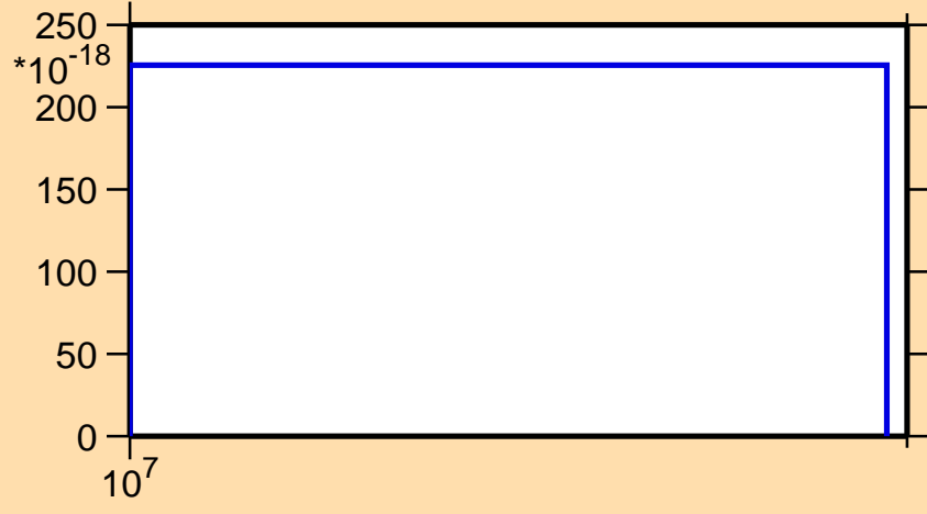
\sigma vs. E for ^{219}\text{Pb} (mt 11)
