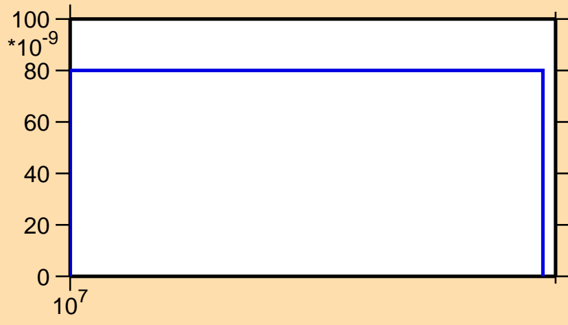
\sigma vs. E for ^{219}\text{Pb}(n,nt)
