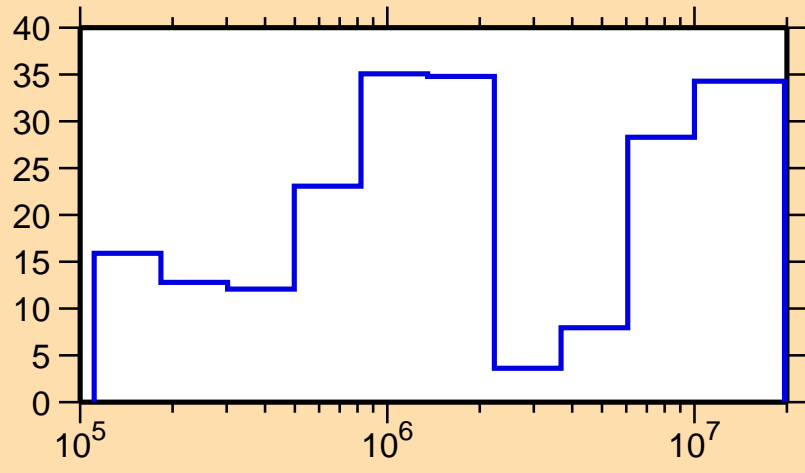
\Delta\sigma/\sigma vs. E for ^{219}\text{Pb}(n,\text{tot.})
