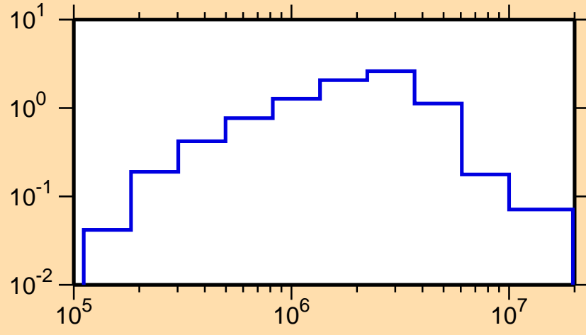
\sigma vs. E for ^{219}\text{Pb}(n,\text{inel.})
