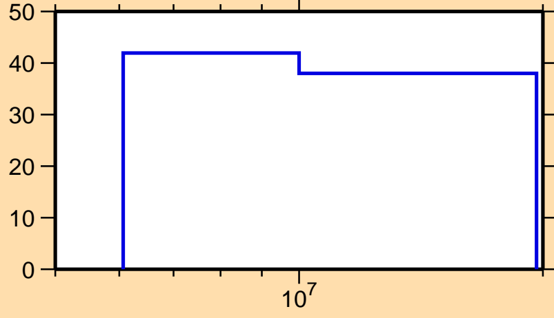
\Delta\sigma/\sigma vs. E for ^{219}\text{Pb}(n,\text{nonel.})
