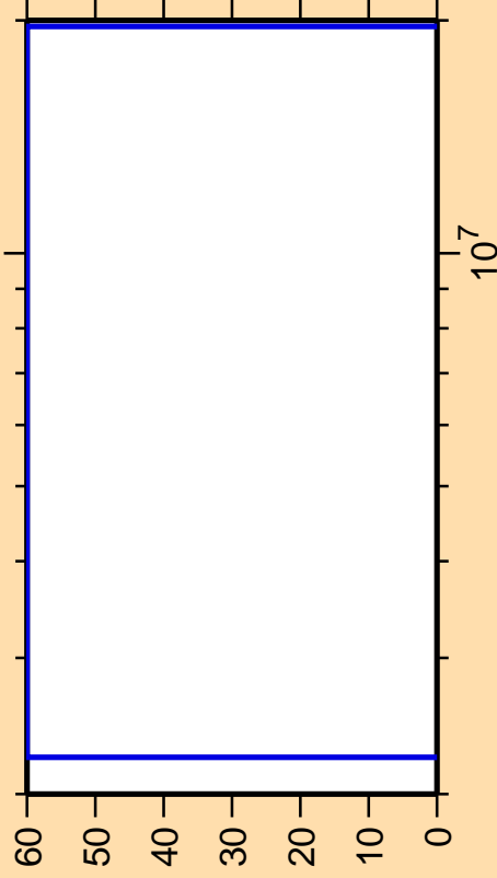
\Delta\sigma/\sigma vs. E for ^{219}\text{Pb}(n,n\text{cont.})
