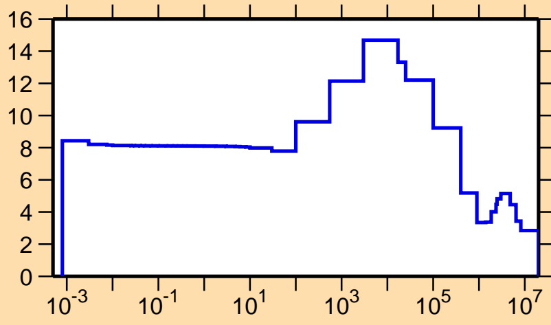
\sigma vs. E for ^{219}\text{Pb}(n,\text{el.})
