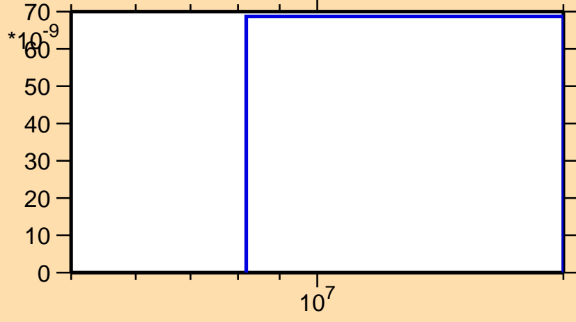
\sigma vs. E for ^{219}\text{Pb}(n,nt)
