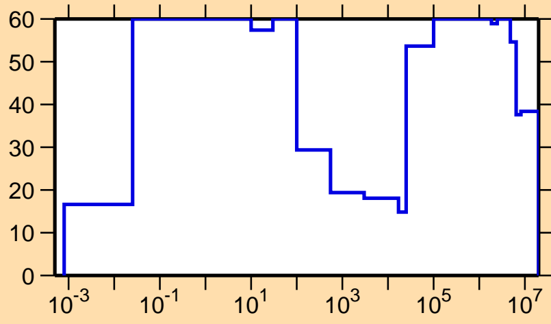
\Delta\sigma/\sigma vs. E for ^{219}\text{Pb}(n,\text{nonel.})
