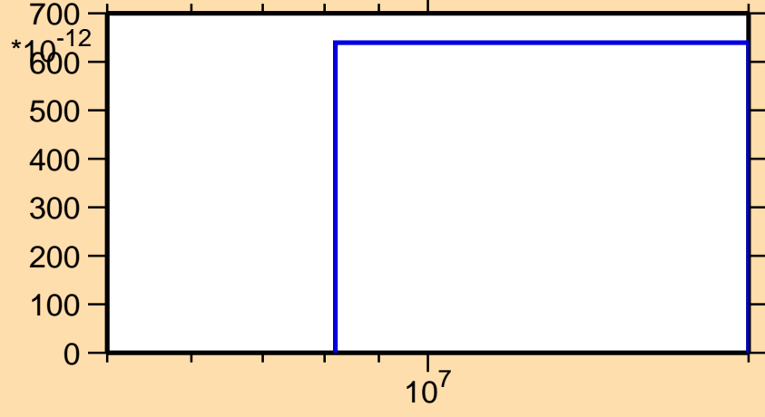
\sigma vs. E for ^{219}\text{Pb}(n,2np)
