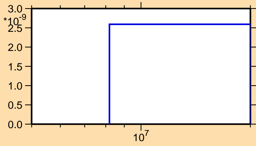
\sigma vs. E for ^{219}\text{Pb}(n,\text{nd})
