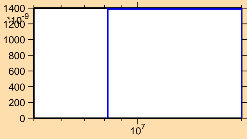
\sigma vs. E for ^{219}\text{Pb}(n,n\alpha)
