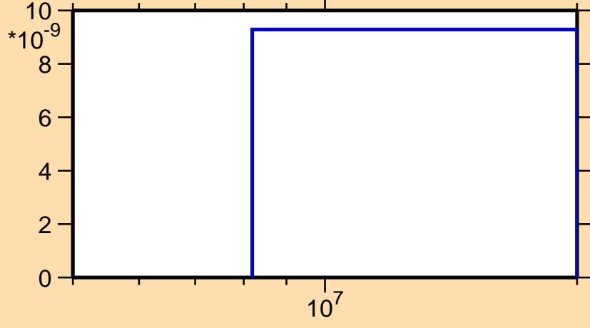
\sigma vs. E for ^{219}\text{Pb}(n,2n\alpha)
