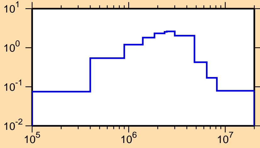
\sigma vs. E for ^{219}\text{Pb}(n,n\text{cont.})
