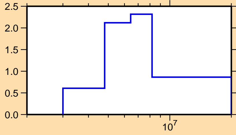
\sigma vs. E for ^{219}\text{Pb}(n,2n)
