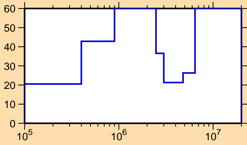
\Delta\sigma/\sigma vs. E for ^{219}\text{Pb}(n,\text{el.})
