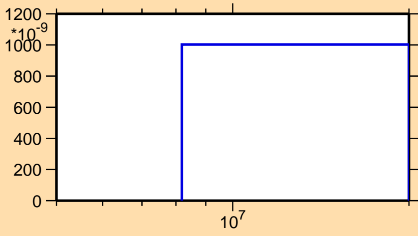
\sigma vs. E for ^{219}\text{Pb}(n,np)
