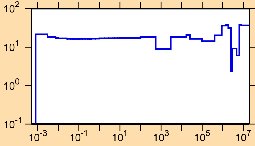
\Delta\sigma/\sigma vs. E for ^{219}\text{Pb}(n,\text{tot.})
