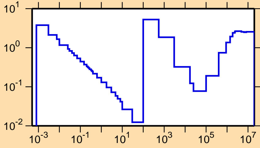
\sigma vs. E for ^{219}\text{Pb}(n,\text{nonel.})
