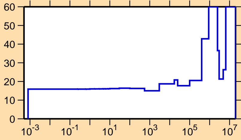
\Delta\sigma/\sigma vs. E for ^{219}\text{Pb}(n,\text{el.})
