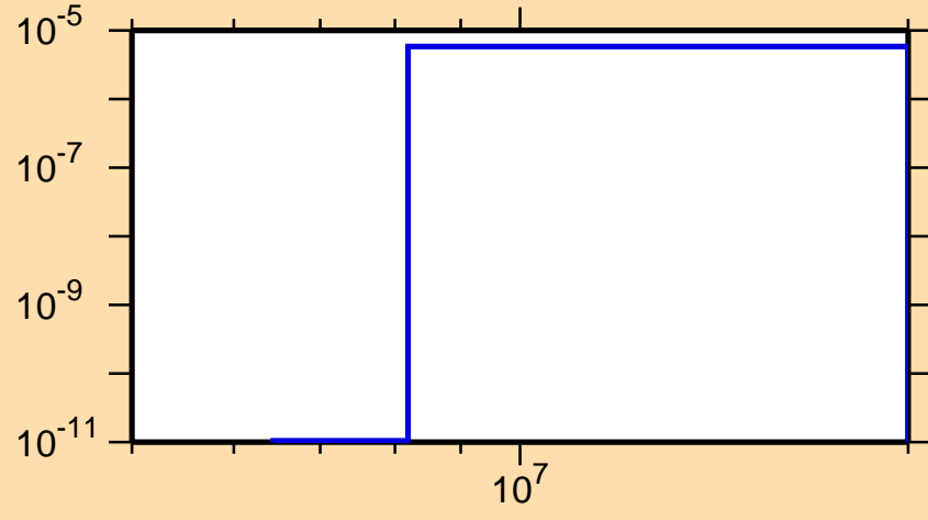
\sigma vs. E for ^{219}\text{Pb}(n,\alpha)
