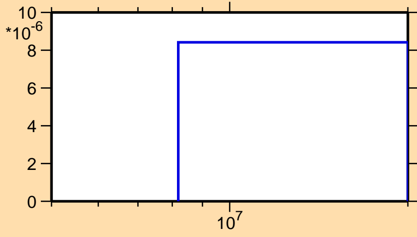
\sigma vs. E for ^{219}\text{Pb}(n,t)
