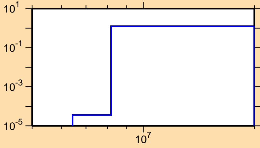
\sigma vs. E for ^{219}\text{Pb}(n,3n)
