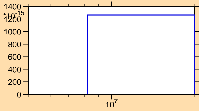
\sigma vs. E for ^{219}\text{Pb}(n,3n\alpha)
