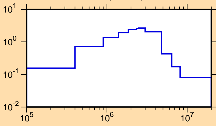
\sigma vs. E for ^{219}\text{Pb}(n,\text{inel.})
