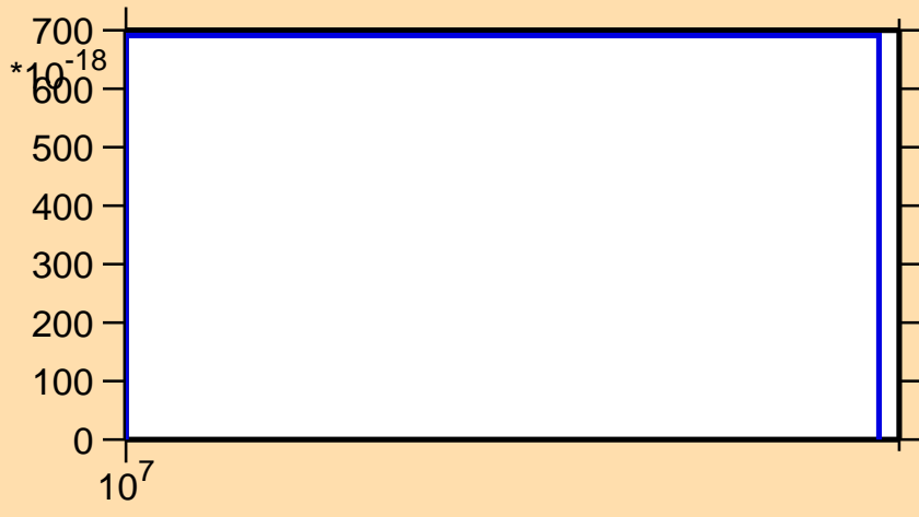
\sigma vs. E for ^{220}\text{Pb} (mt 11)
