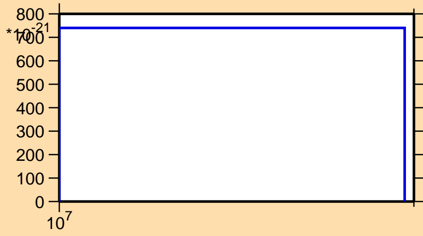
\sigma vs. E for ^{220}\text{Pb} (mt 42)
