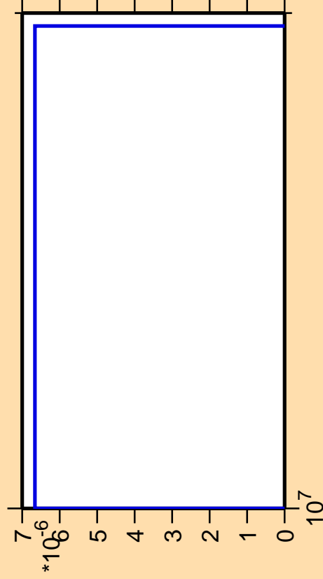
\Delta\sigma/\sigma vs. E for ^{220}\text{Pb} (mt 42)
