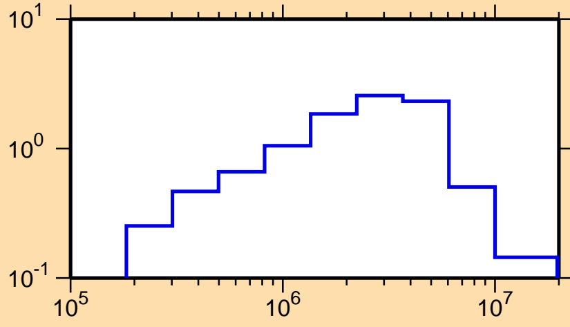
\sigma vs. E for ^{220}\text{Pb}(n,\text{inel.})
