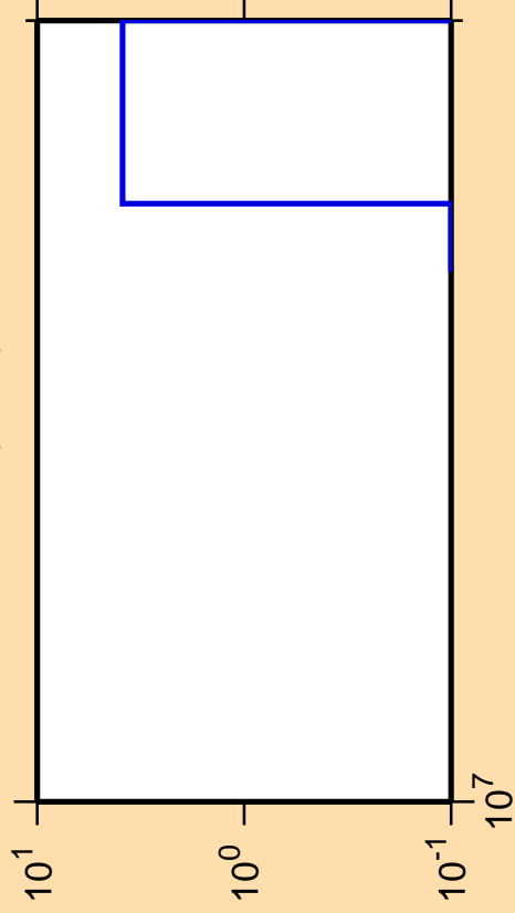
\Delta\sigma/\sigma vs. E for ^{92}\text{Pd}(n,nd)
