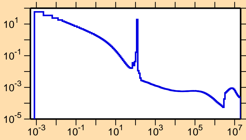
\sigma vs. E for ^{92}\text{Pd}(n,\gamma)
