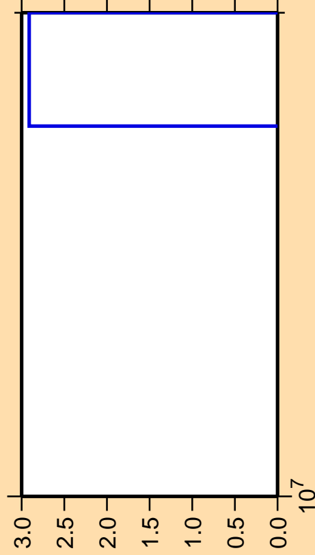
\Delta\sigma/\sigma vs. E for ^{92}\text{Pd}(n,2np)
