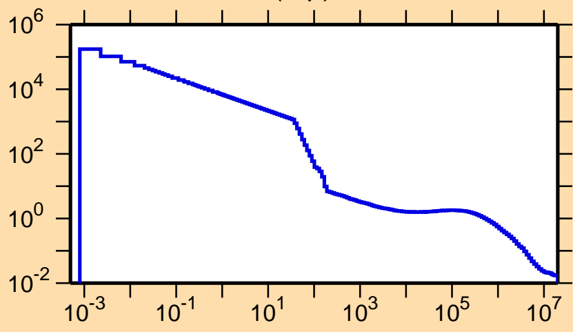
\sigma vs. E for ^{92}\text{Pd}(n,p)
