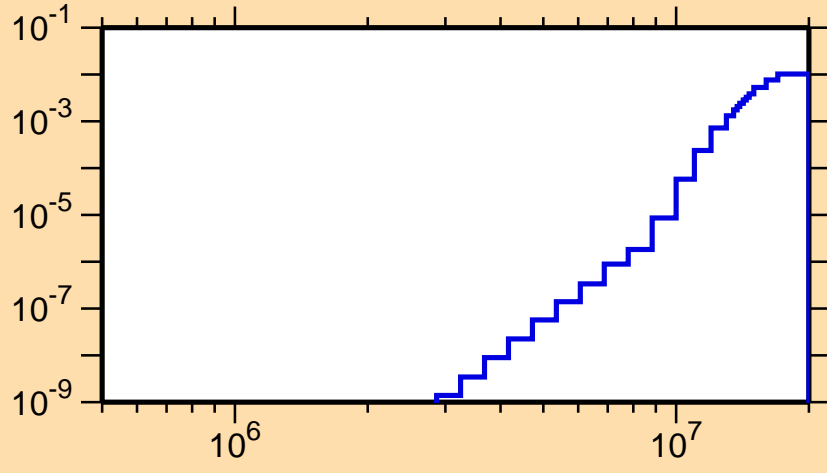
\sigma vs. E for ^{92}\text{Pd}(n,\text{He}3)
