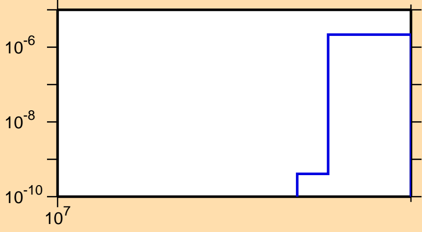
\sigma vs. E for ^{92}\text{Pd}(n,2n)
