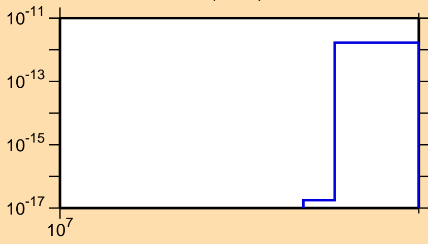
\sigma vs. E for ^{92}\text{Pd}(n,nd)
