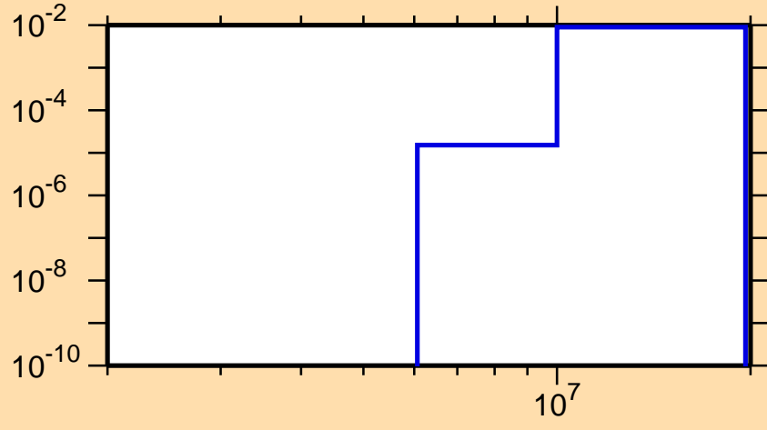
\sigma vs. E for ^{92}\text{Pd}(n,\text{pd})
