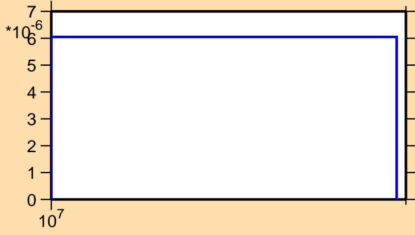
\sigma vs. E for ^{92}\text{Pd}(n,t)
