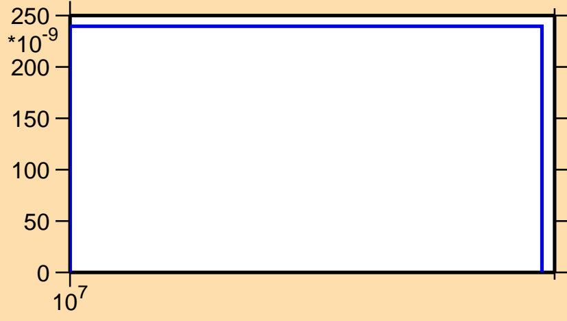
\sigma vs. E for ^{92}\text{Pd}(n,\text{pt})
