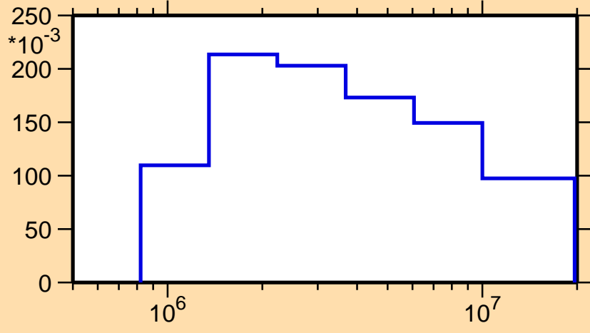
\sigma vs. E for ^{92}\text{Pd}(n,n_1)
