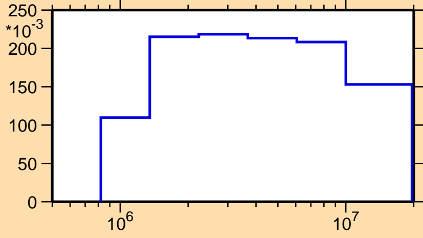
\sigma vs. E for ^{92}\text{Pd}(n,\text{inel.})
