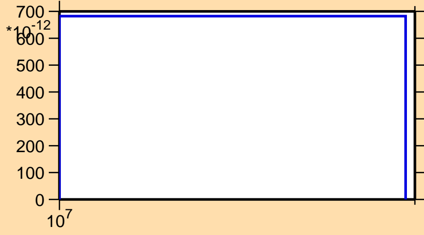
\sigma vs. E for ^{92}\text{Pd}(\text{mt } 45)
