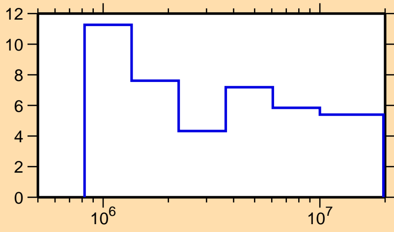
\Delta\sigma/\sigma vs. E for ^{92}\text{Pd}(n,\text{nonel.})
