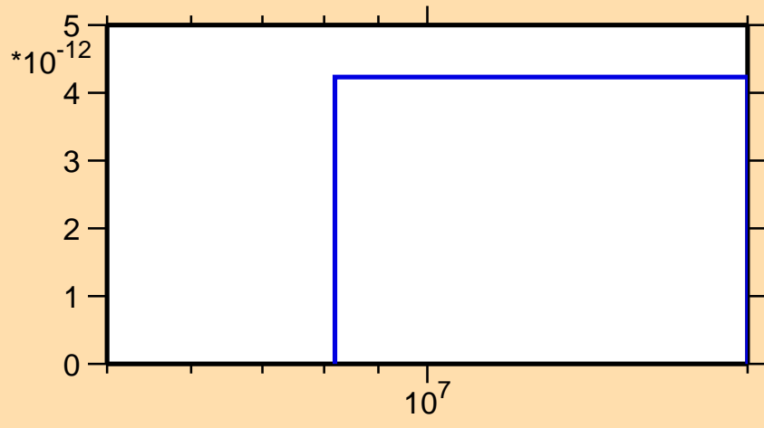
\sigma vs. E for ^{92}\text{Pd}(\text{mt117})
