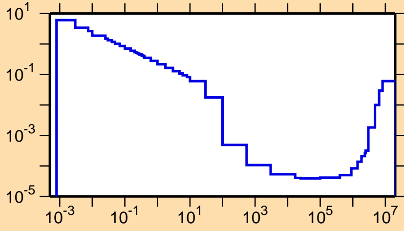
\sigma vs. E for ^{92}\text{Pd}(n,\alpha)
