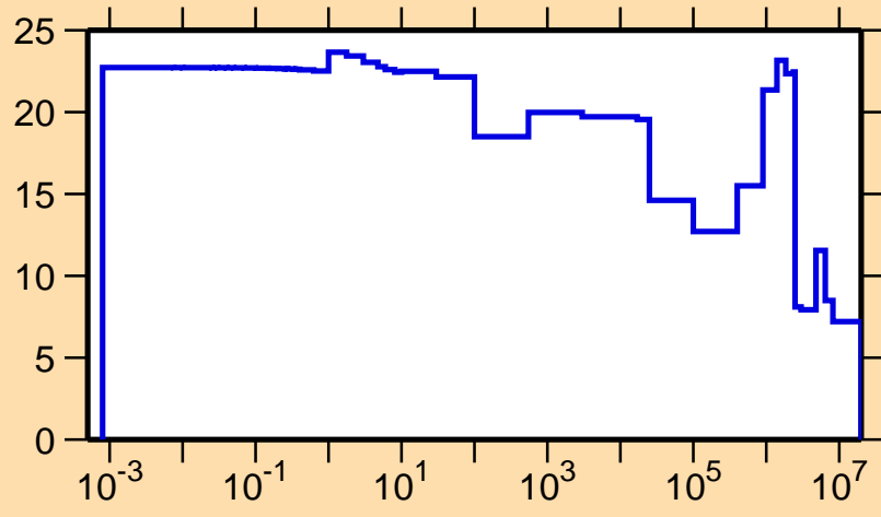
\Delta\sigma/\sigma vs. E for ^{92}\text{Pd}(n,el.)
