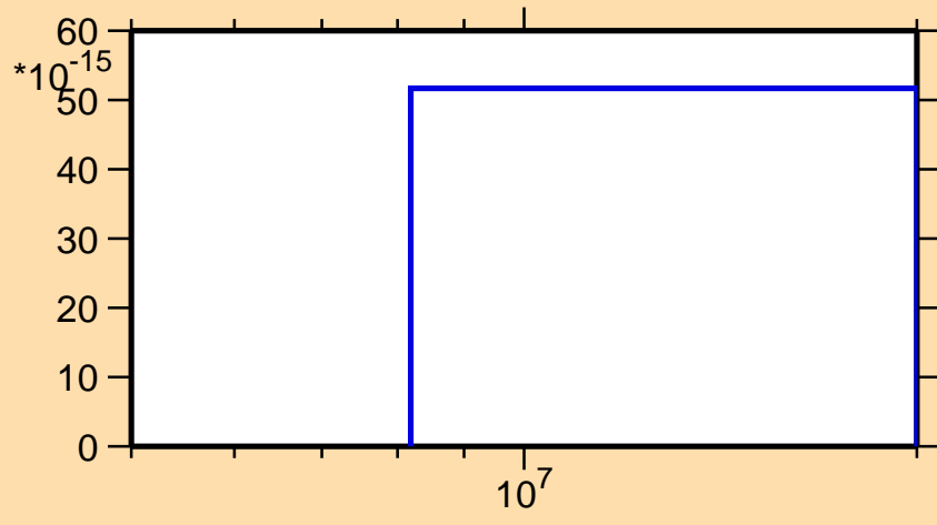
\sigma vs. E for ^{92}\text{Pd}(n,2np)
