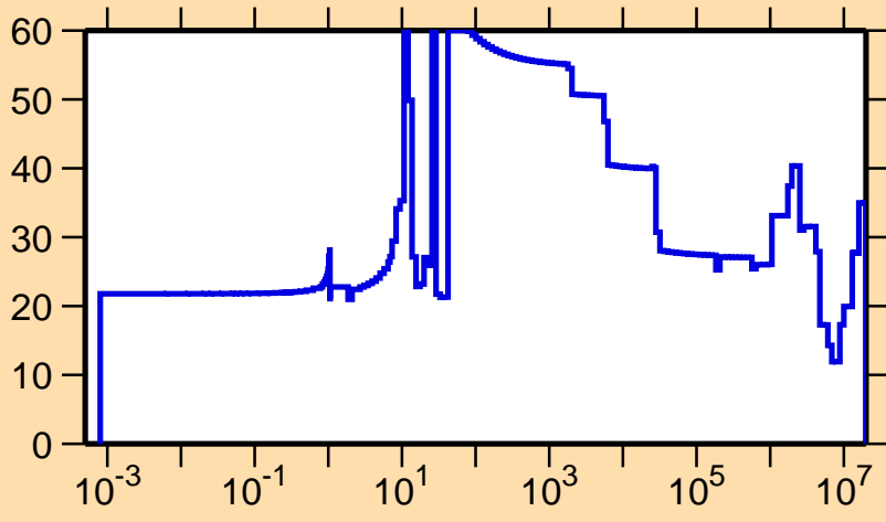
\Delta\sigma/\sigma vs. E for ^{93}\text{Pd}(n,el.)
