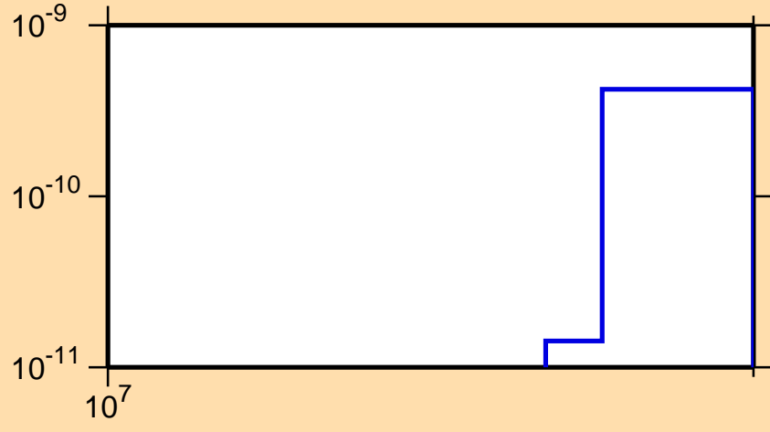
\sigma vs. E for ^{93}\text{Pd}(\text{mt117})
