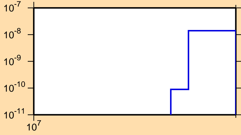
\sigma vs. E for ^{93}\text{Pd}(n,\text{nd})
