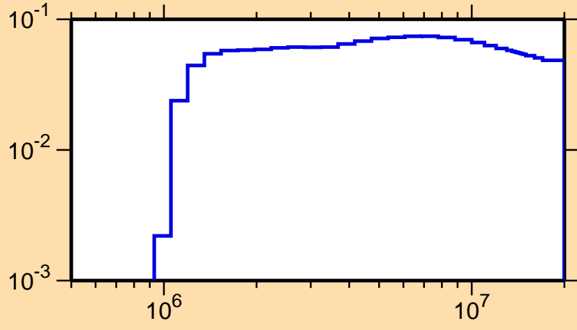
\sigma vs. E for ^{93}\text{Pd}(n,\text{inel.})
