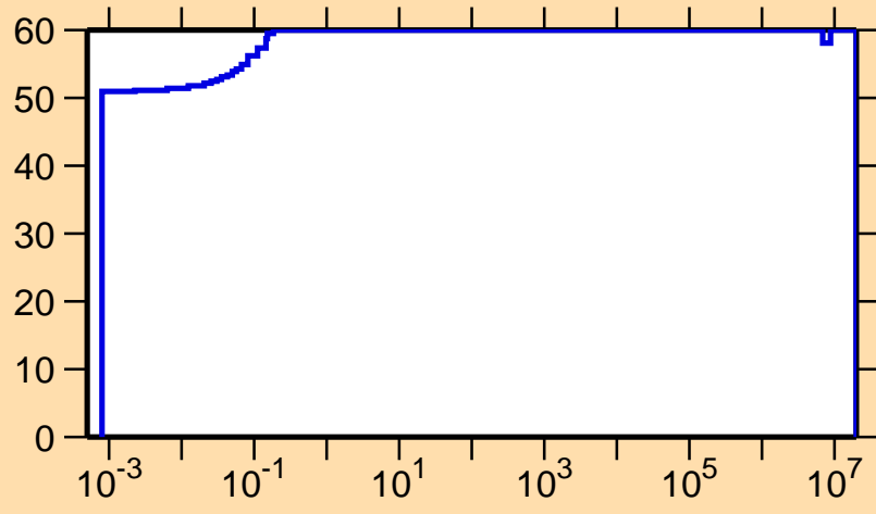
\Delta\sigma/\sigma vs. E for ^{93}\text{Pd}(n,\gamma)
