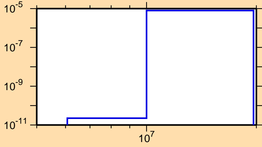
\sigma vs. E for ^{93}\text{Pd}(n,n\alpha)
