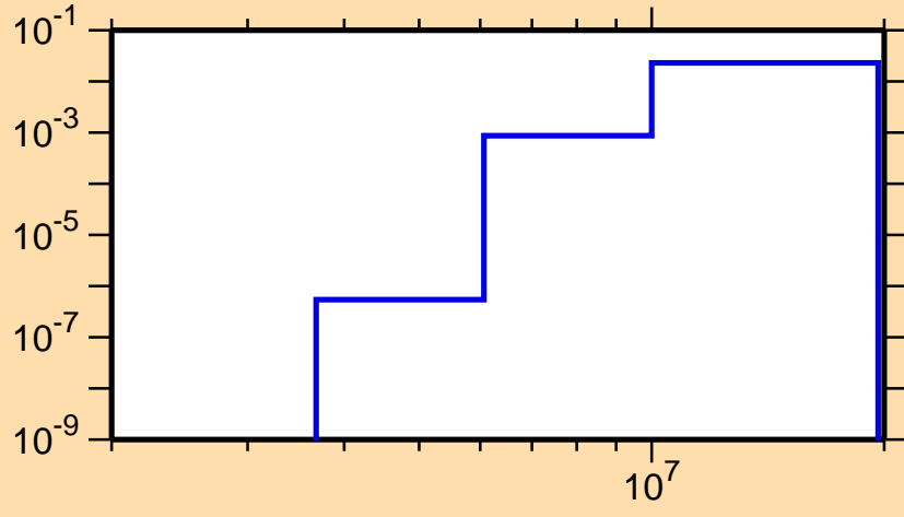
\sigma vs. E for ^{93}\text{Pd}(n,d)
