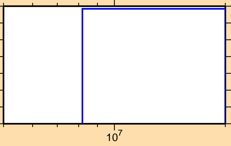
\sigma vs. E for ^{93}\text{Pd}(n,t)
