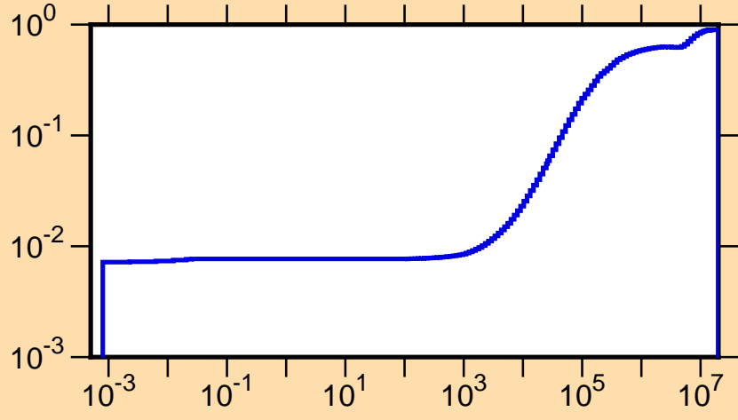
\mu vs. E for ^{94}\text{Pd}(\text{mt251})
