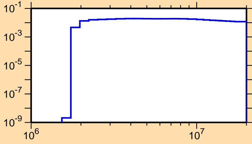
\sigma vs. E for ^{94}\text{Pd}(n,n_2)
