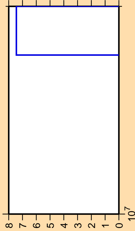
\Delta\sigma/\sigma vs. E for ^{94}\text{Pd}(n,2np)
