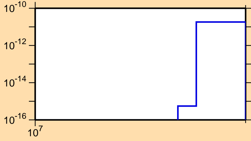
\sigma vs. E for ^{94}\text{Pd}(n,\text{nd})
