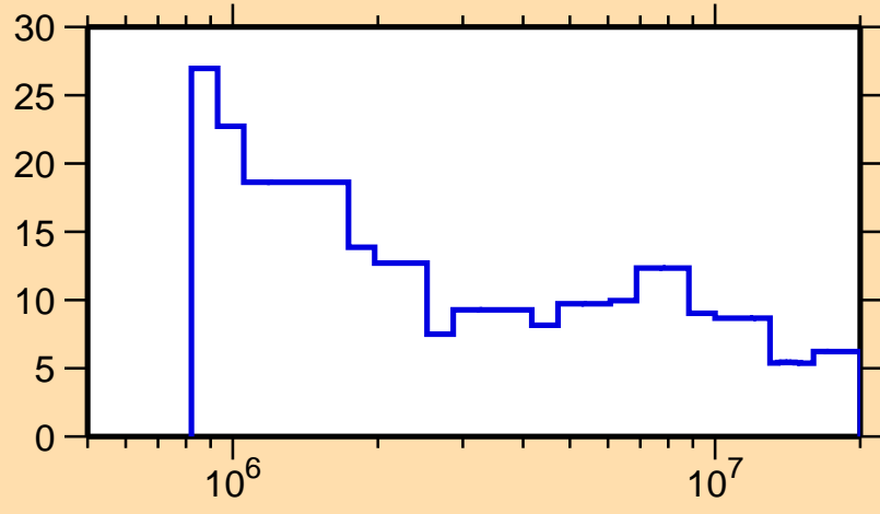
\Delta\sigma/\sigma vs. E for ^{94}\text{Pd}(n,\text{tot.})
