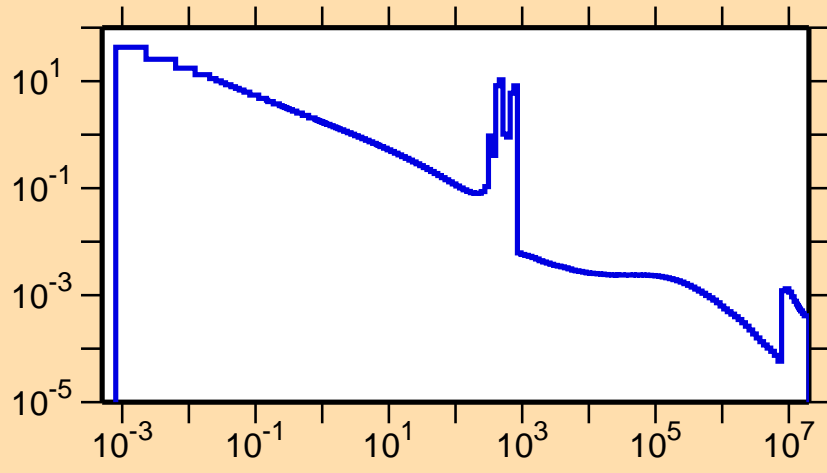
\sigma vs. E for ^{94}\text{Pd}(n,\gamma)
