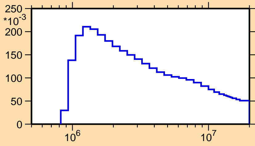
\sigma vs. E for ^{94}\text{Pd}(n,n_1)
