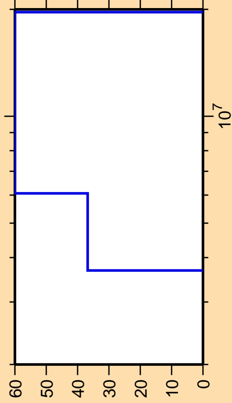
\Delta\sigma/\sigma vs. E for ^{94}\text{Pd}(n,np)
