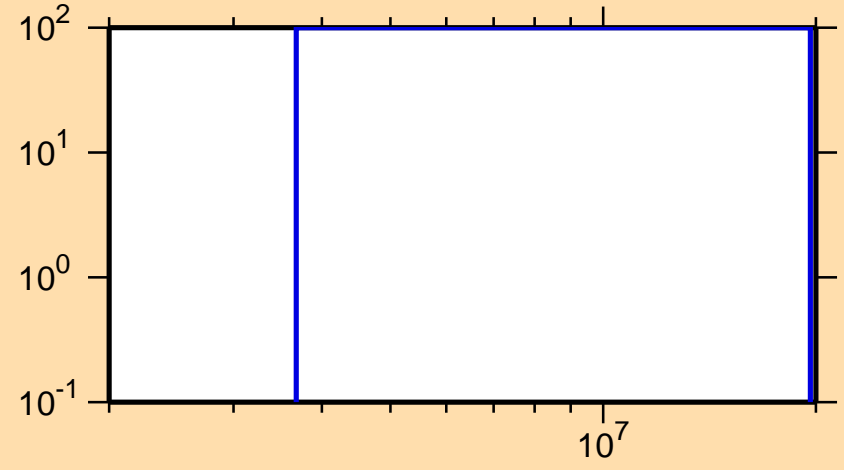
\Delta\sigma/\sigma vs. E for ^{94}\text{Pd}(n,ncont.)
