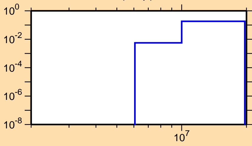
\sigma vs. E for ^{94}\text{Pd}(n,np)
