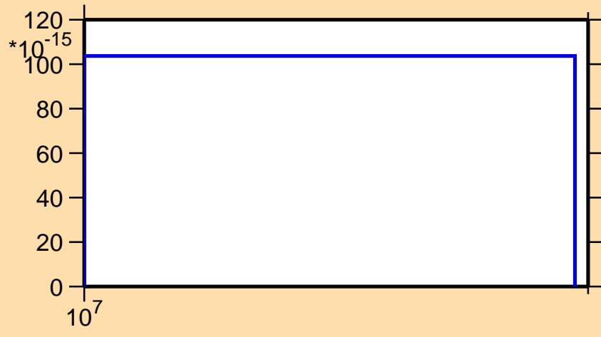
\sigma vs. E for ^{94}\text{Pd}(n,nd)
