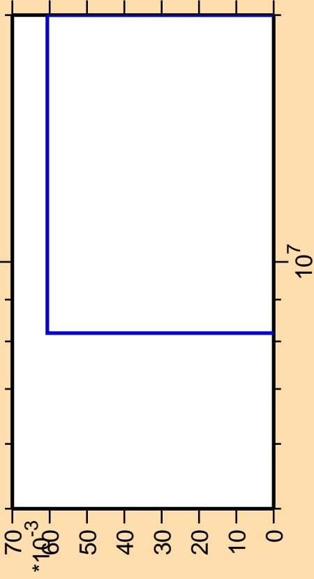
\Delta\sigma/\sigma vs. E for ^{94}\text{Pd}(n,2np)
