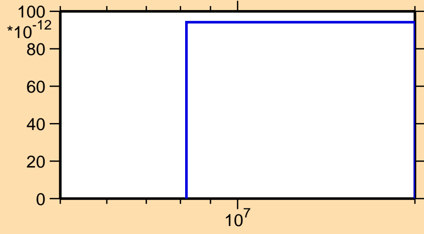
\sigma vs. E for ^{94}\text{Pd}(\text{mt } 45)
