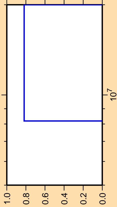
\Delta\sigma/\sigma vs. E for ^{94}\text{Pd}(n,nd)
