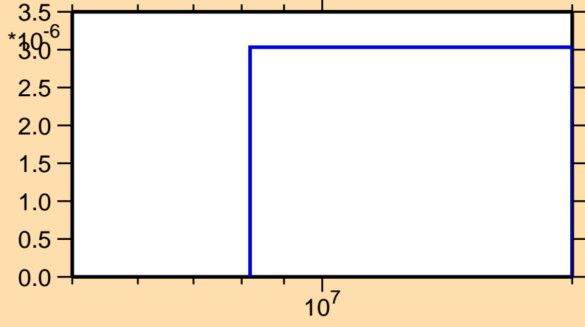
\sigma vs. E for ^{94}\text{Pd}(n,t)
