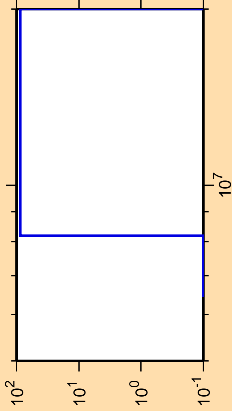
\Delta\sigma/\sigma vs. E for ^{94}\text{Pd}(n,n\alpha)
