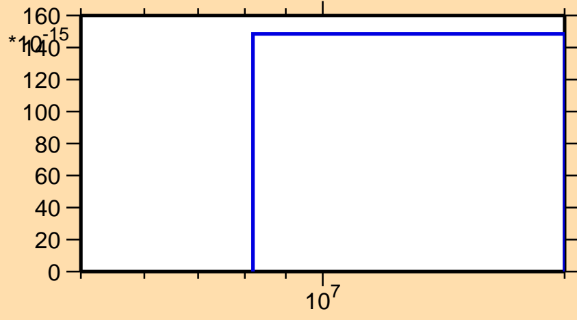
\sigma vs. E for ^{94}\text{Pd}(n,nd)
