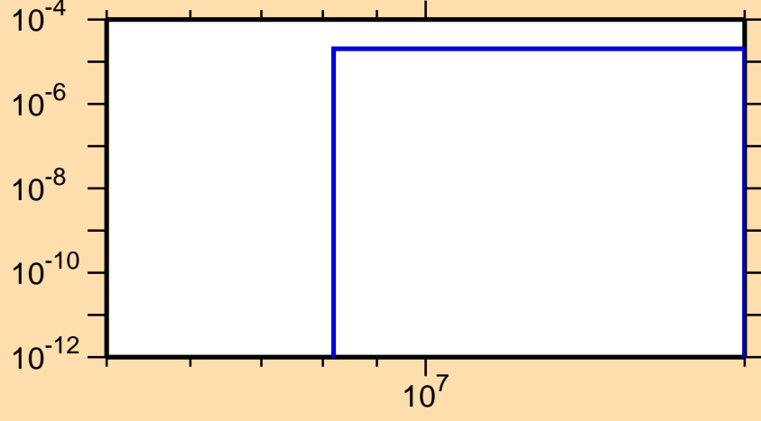
\sigma vs. E for ^{94}\text{Pd}(n,n\alpha)
