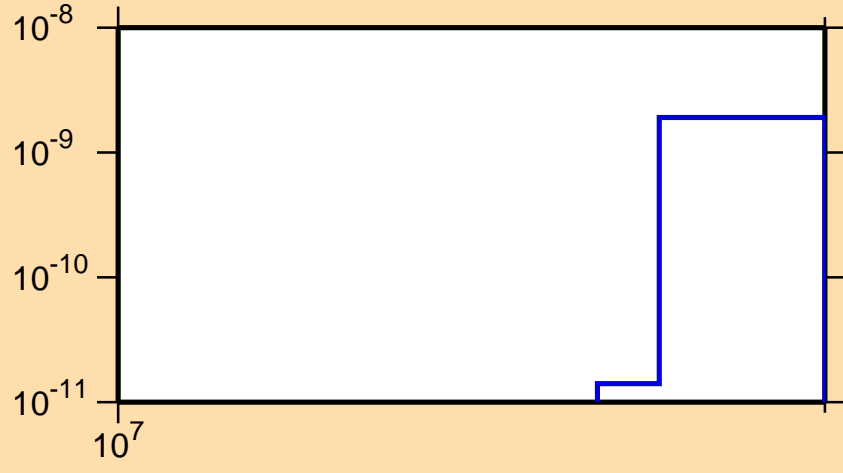
\sigma vs. E for ^{95}\text{Pd}(\text{mt } 34)
