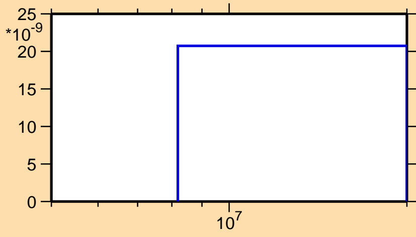
\sigma vs. E for ^{95}\text{Pd}(n,2np)
