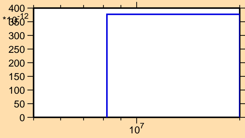
\sigma vs. E for ^{95}\text{Pd}(n,nd)
