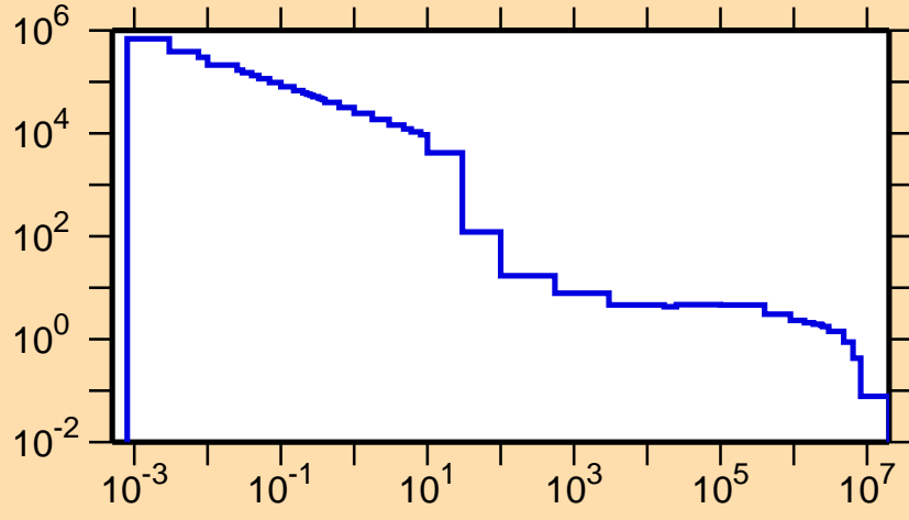
\sigma vs. E for ^{95}\text{Pd}(n,p)
