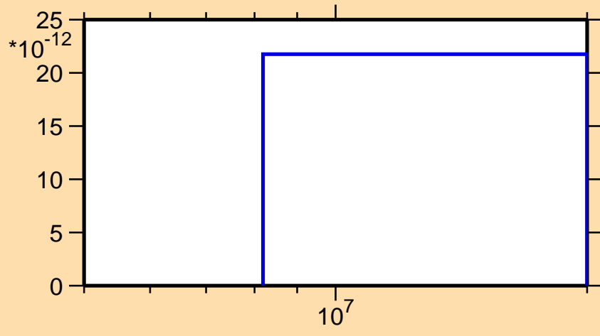
\sigma vs. E for ^{95}\text{Pd}(\text{mt } 45)
