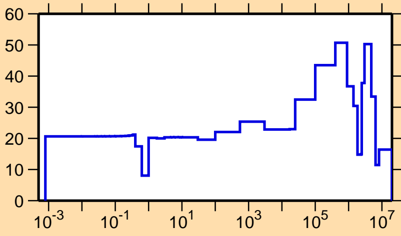
\Delta\sigma/\sigma vs. E for ^{95}\text{Pd}(n,el.)
