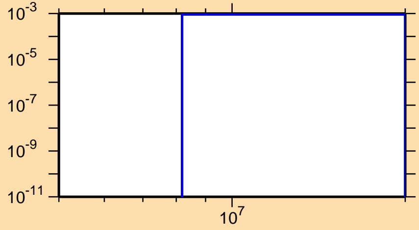
\sigma vs. E for ^{95}\text{Pd}(n,\text{pd})
