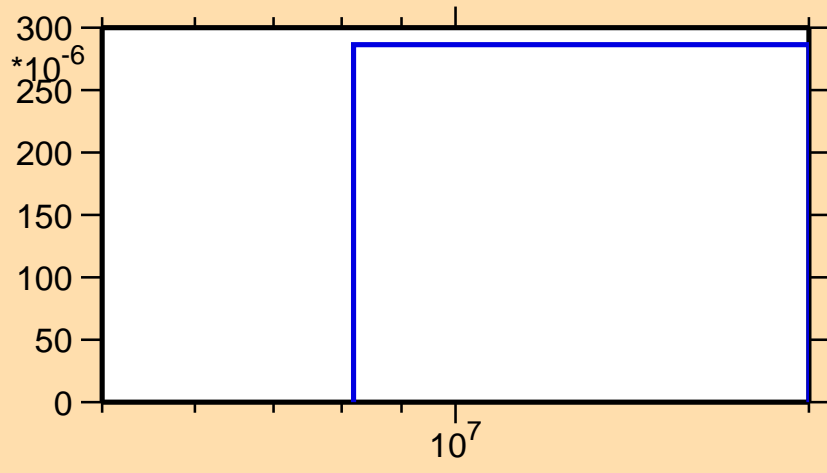
\sigma vs. E for ^{95}\text{Pd}(n,2n)
