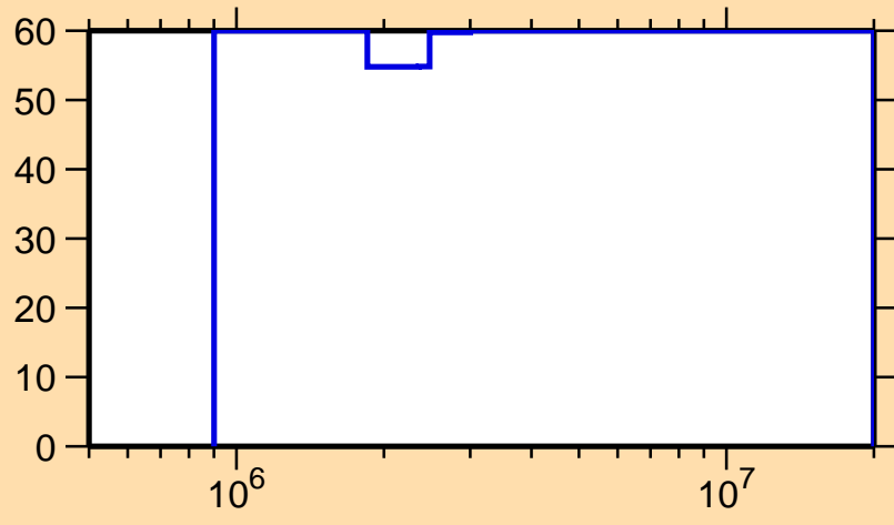
\Delta\sigma/\sigma vs. E for ^{95}\text{Pd}(n,n_1)
