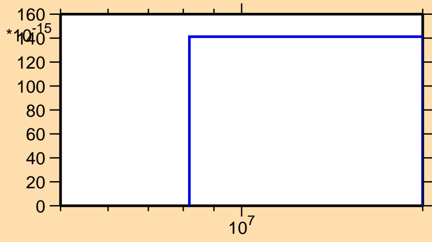
\sigma vs. E for ^{95}\text{Pd}(\text{mt117})
