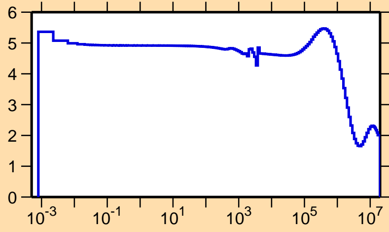
\sigma vs. E for ^{95}\text{Pd}(n,\text{el.})
