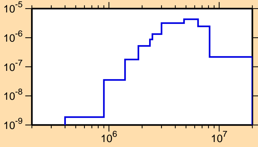
\sigma vs. E for ^{95}\text{Pd}(n,n_4)
