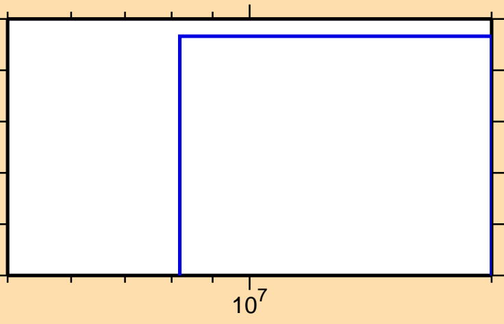
\sigma vs. E for ^{95}\text{Pd}(n,2np)
