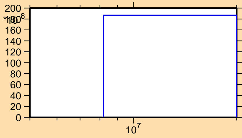
\sigma vs. E for ^{95}\text{Pd}(n,t)
