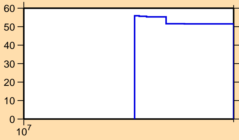
\Delta\sigma/\sigma vs. E for ^{96}\text{Pd}(n,\text{inel.})
