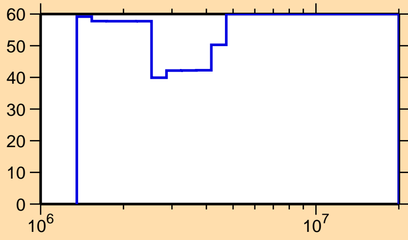
\Delta\sigma/\sigma vs. E for ^{96}\text{Pd}(n,n_1)
