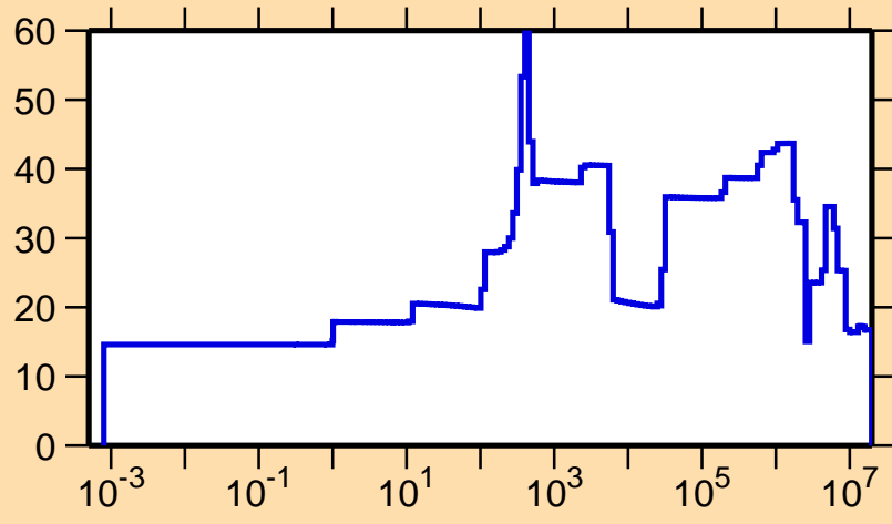
\Delta\sigma/\sigma vs. E for ^{96}\text{Pd}(n,\text{el.})
