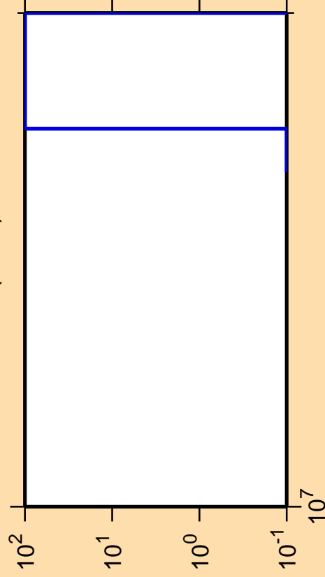
\Delta\sigma/\sigma vs. E for ^{96}\text{Pd}(n,\text{nd})
