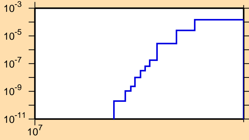
\sigma vs. E for ^{96}\text{Pd}(n,t)
