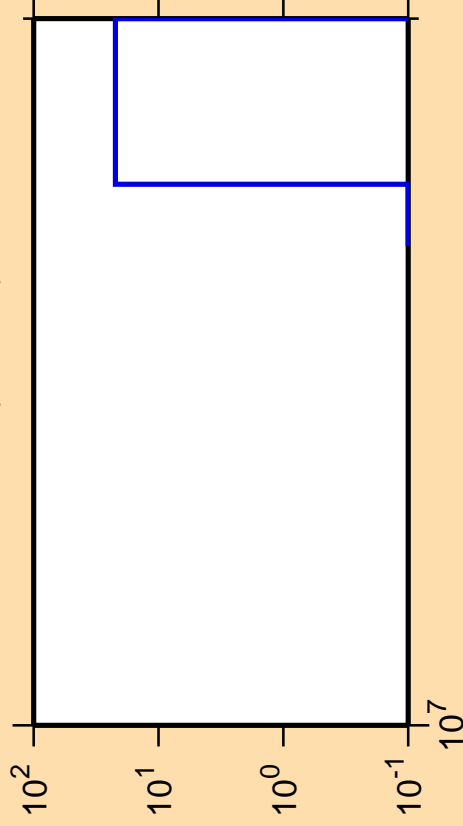
\Delta\sigma/\sigma vs. E for ^{96}\text{Pd}(\text{mt117})
