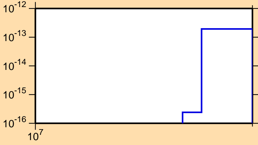
\sigma vs. E for ^{96}\text{Pd}(\text{mt } 34)
