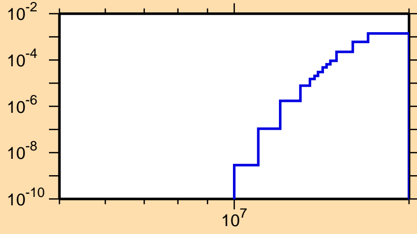
\sigma vs. E for ^{96}\text{Pd}(n,n\alpha)
