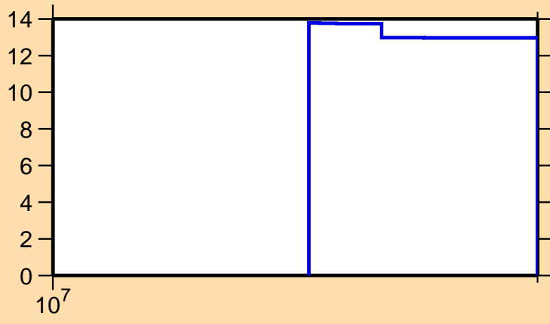
\Delta\sigma/\sigma vs. E for ^{96}\text{Pd}(n,\text{nonel.})
