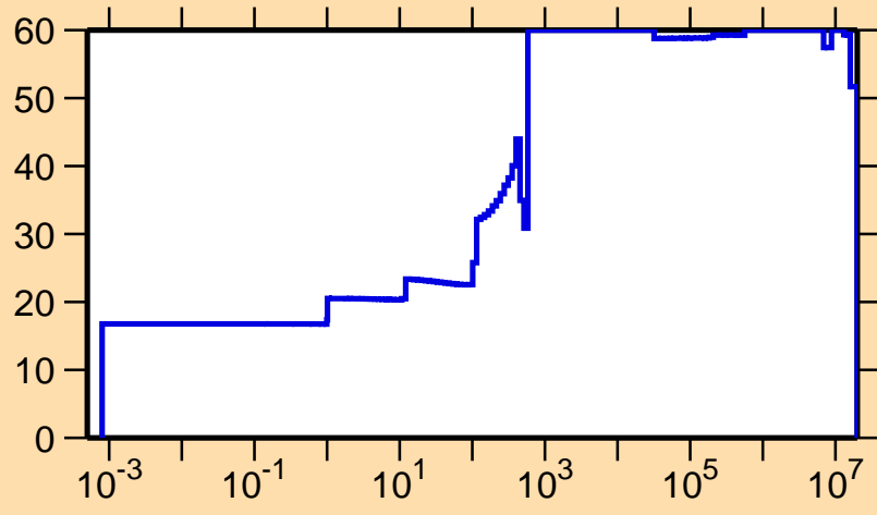
\Delta\sigma/\sigma vs. E for ^{96}\text{Pd}(n,\gamma)
