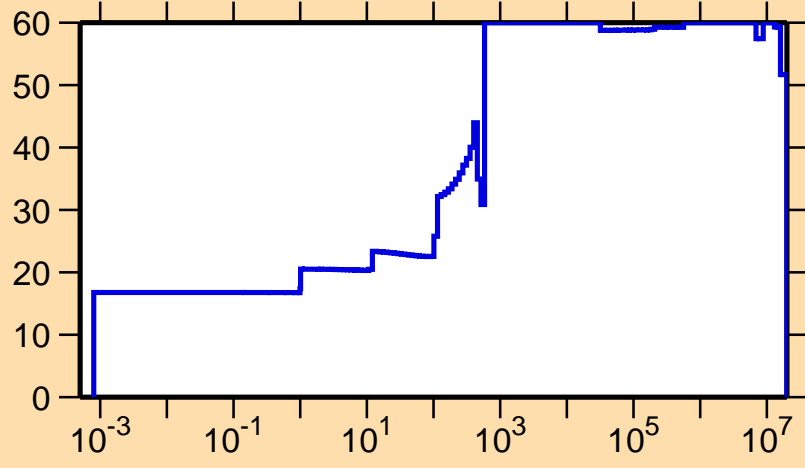
\Delta\sigma/\sigma vs. E for ^{96}\text{Pd}(n,\gamma)
