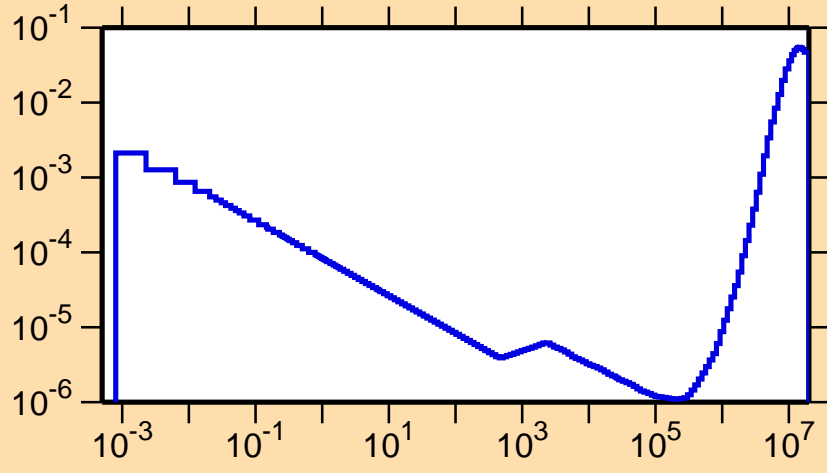
\sigma vs. E for ^{96}\text{Pd}(n,\alpha)
