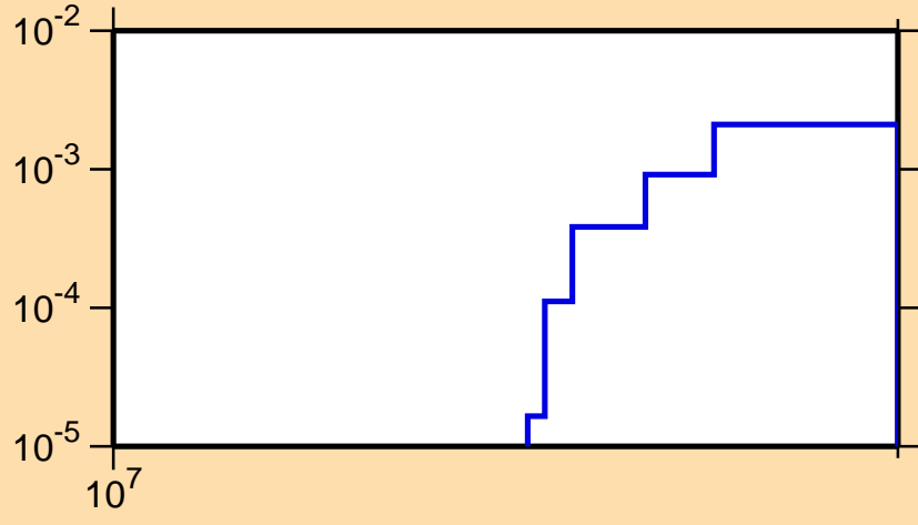
\sigma vs. E for ^{96}\text{Pd}(n,2n)
