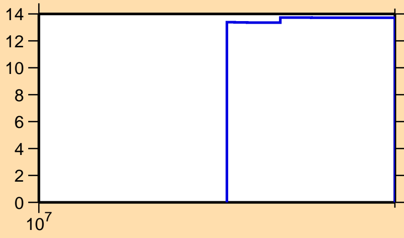
\Delta\sigma/\sigma vs. E for ^{96}\text{Pd}(n,\text{tot.})
