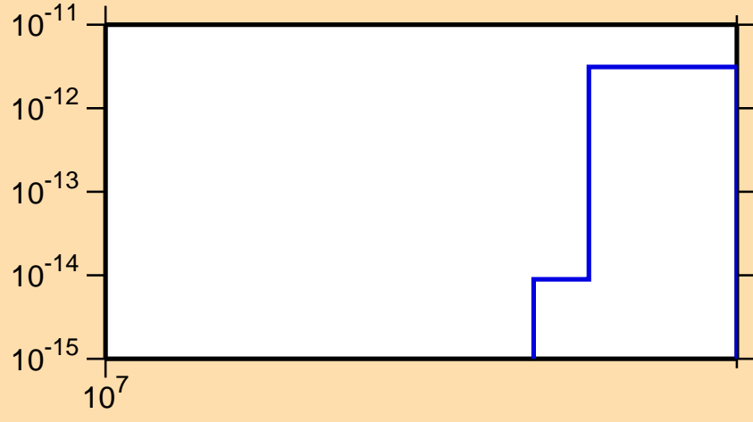
\sigma vs. E for ^{96}\text{Pd}(\text{mt117})
