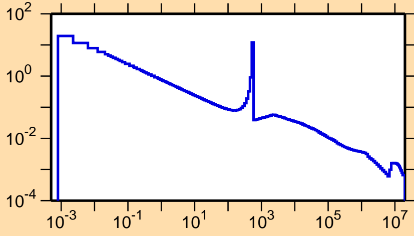
\sigma vs. E for ^{96}\text{Pd}(n,\gamma)
