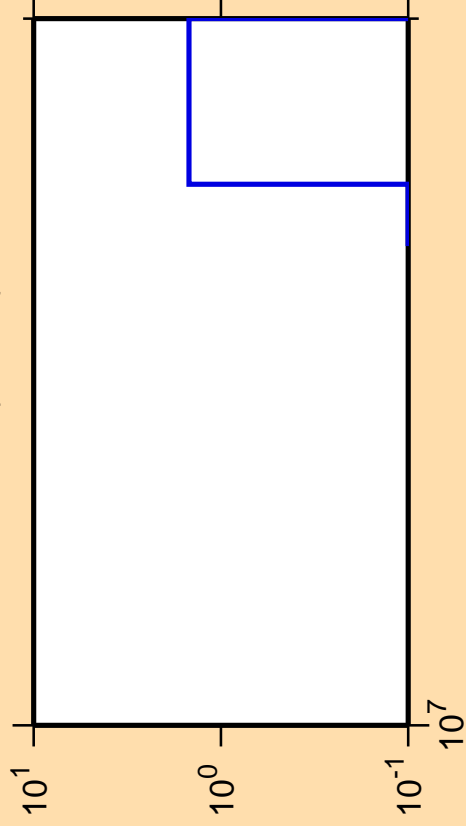
\Delta\sigma/\sigma vs. E for ^{96}\text{Pd}(\text{mt } 34)
