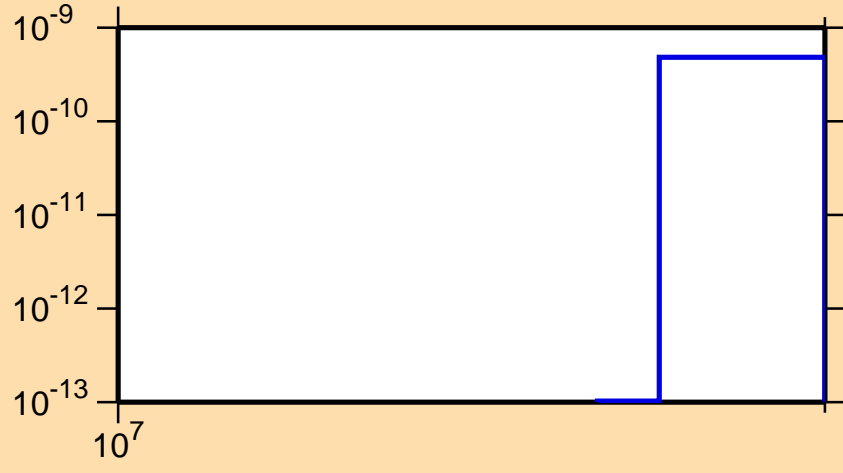
\sigma vs. E for ^{96}\text{Pd}(\text{mt } 45)
