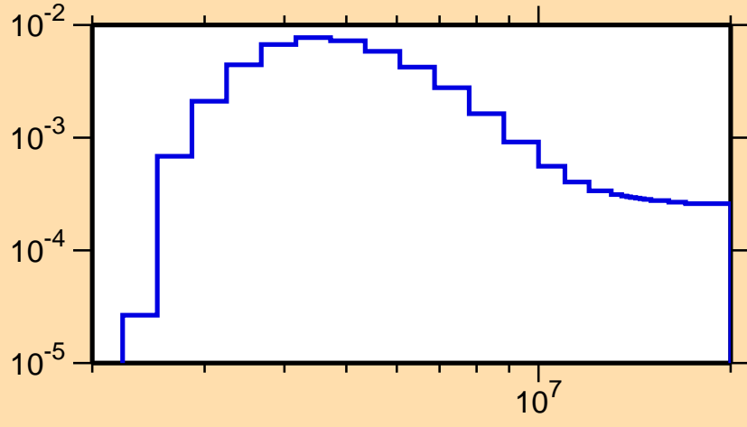
\sigma vs. E for ^{96}\text{Pd}(n,n_4)
