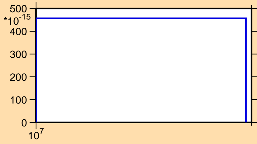
\sigma vs. E for ^{96}\text{Pd}(n,nd)
