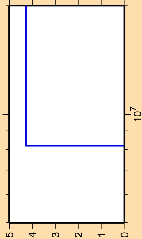
\Delta\sigma/\sigma vs. E for ^{96}\text{Pd}(n,nd)
