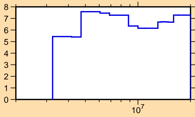
\Delta\sigma/\sigma vs. E for ^{98}\text{Pd}(n,n\text{onel.})
