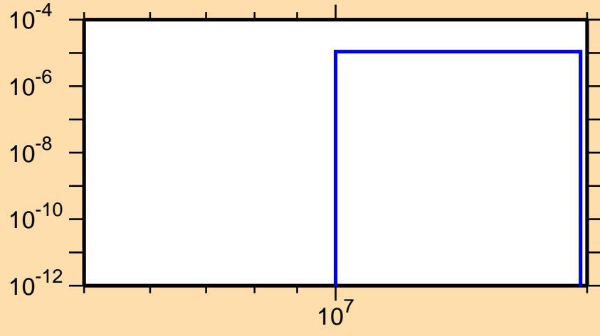
\sigma vs. E for ^{98}\text{Pd}(n,pd)
