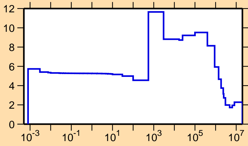
\sigma vs. E for ^{98}\text{Pd}(n,\text{el.})
