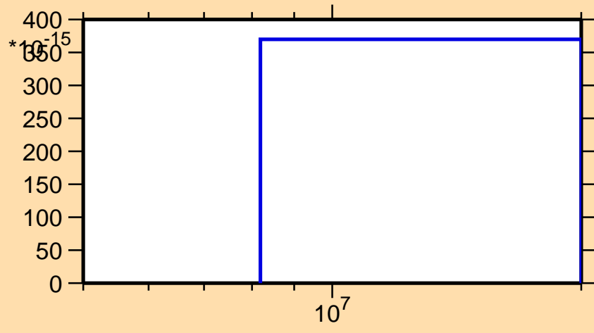
\sigma vs. E for ^{98}\text{Pd}(\text{mt } 34)
