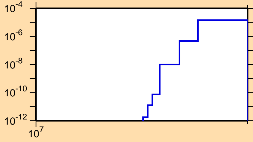
\sigma vs. E for ^{99}\text{Pd}(n,2n\alpha)
