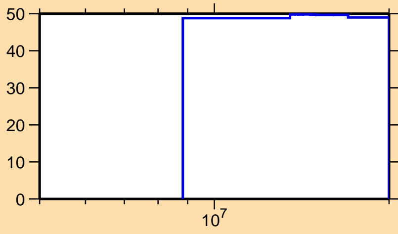
\Delta\sigma/\sigma vs. E for ^{99}\text{Pd}(n,2n)
