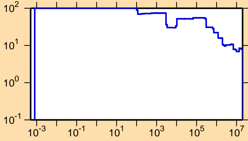
\Delta\sigma/\sigma vs. E for ^{99}\text{Pd}(n,\text{nonel.})
