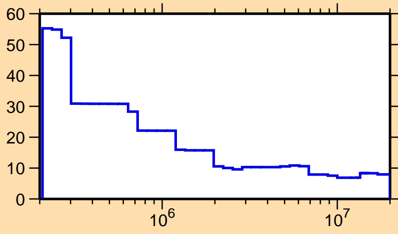
\Delta\sigma/\sigma vs. E for ^{99}\text{Pd}(n,\text{nonel.})
