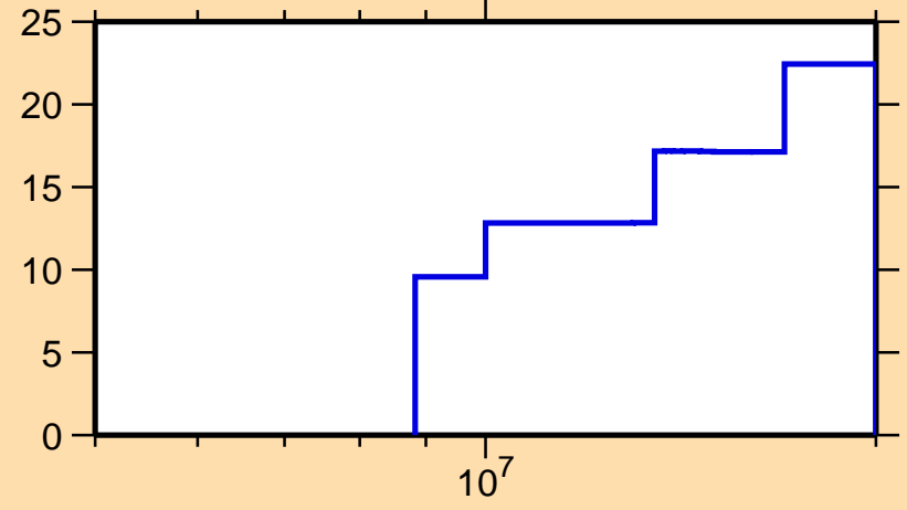
\Delta\sigma/\sigma vs. E for ^{99}\text{Pd}(n,\text{el.})
