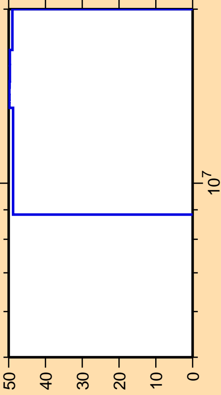
\Delta\sigma/\sigma vs. E for ^{99}\text{Pd}(n,2n)
