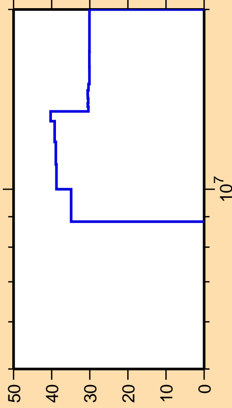
\Delta\sigma/\sigma vs. E for ^{99}\text{Pd}(n,n\text{cont.})
