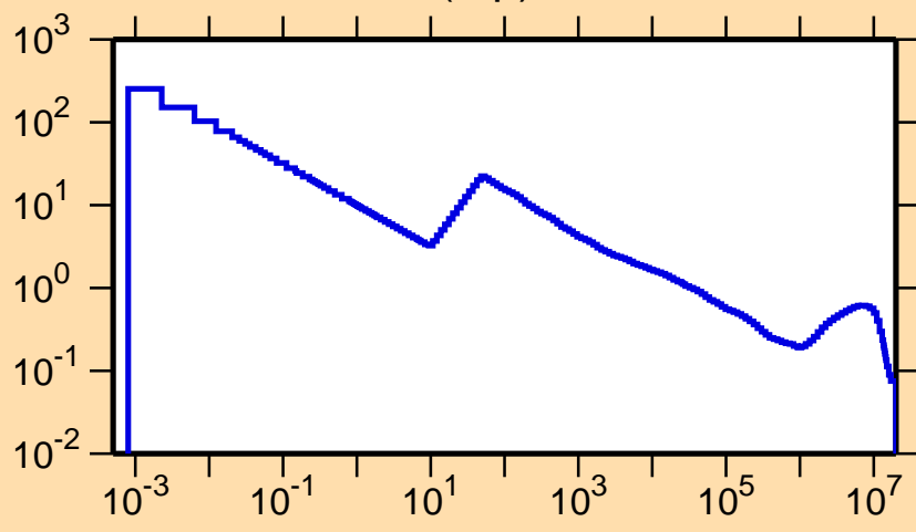
\sigma vs. E for ^{99}\text{Pd}(n,p)
