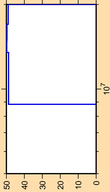
\Delta\sigma/\sigma vs. E for ^{99}\text{Pd}(n,2n)
