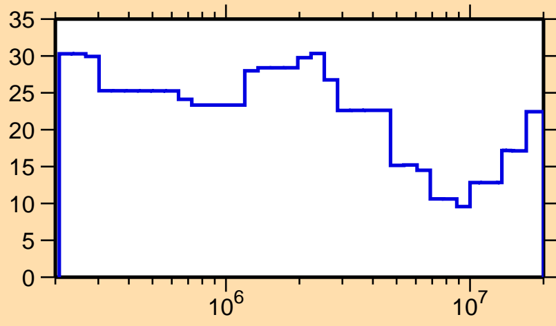
\Delta\sigma/\sigma vs. E for ^{99}\text{Pd}(n,\text{el.})
