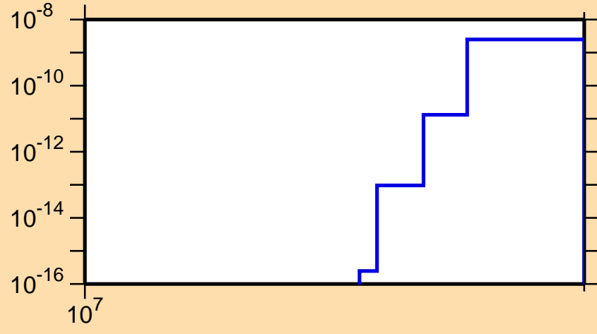
\sigma vs. E for ^{99}\text{Pd}(\text{mt } 34)
