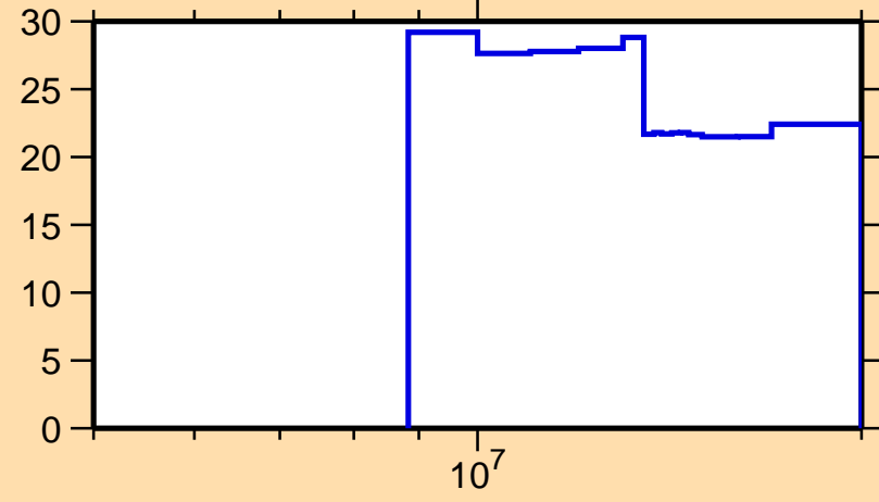
\Delta\sigma/\sigma vs. E for ^{99}\text{Pd}(n,\text{inel.})
