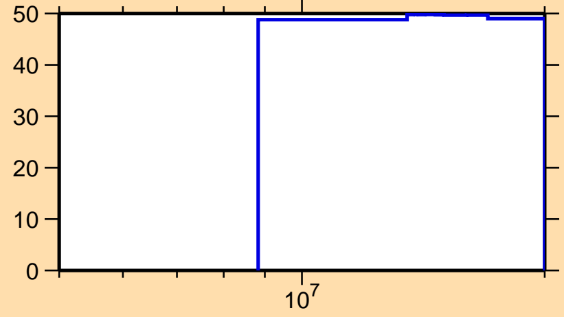
\Delta\sigma/\sigma vs. E for ^{99}\text{Pd}(n,2n)
