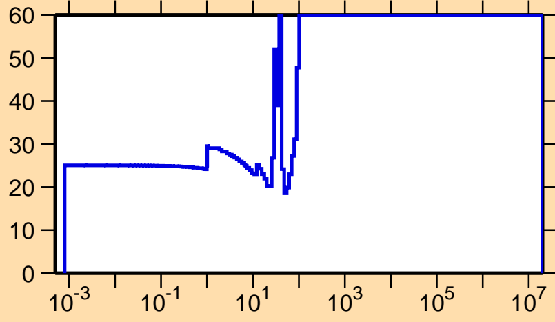
\Delta\sigma/\sigma vs. E for ^{99}\text{Pd}(n,\gamma)
