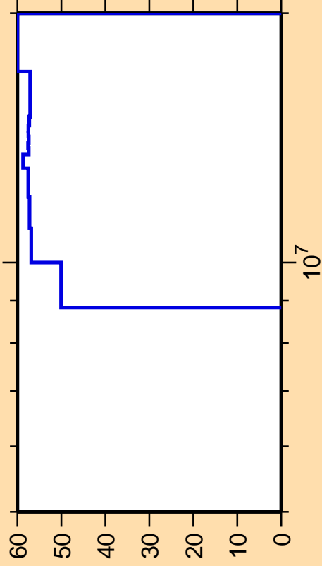
\Delta\sigma/\sigma vs. E for ^{99}\text{Pd}(n,n_1)
