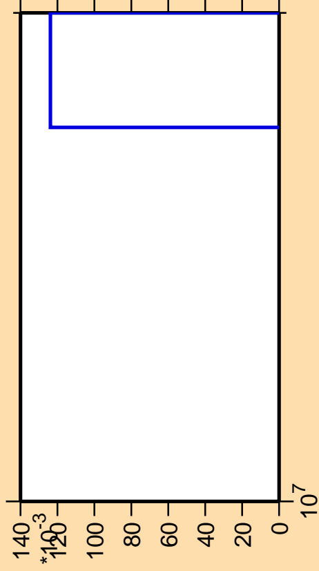
\Delta\sigma/\sigma vs. E for ^{99}\text{Pd}(n,nt)
