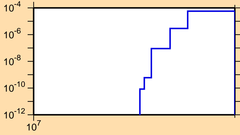
\sigma vs. E for ^{99}\text{Pd}(n,\text{nd})
