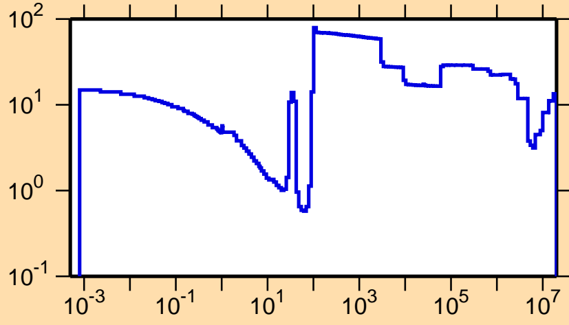
\Delta\sigma/\sigma vs. E for ^{99}\text{Pd}(n,\text{tot.})
