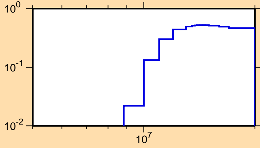
\sigma vs. E for ^{99}\text{Pd}(n,2n)
