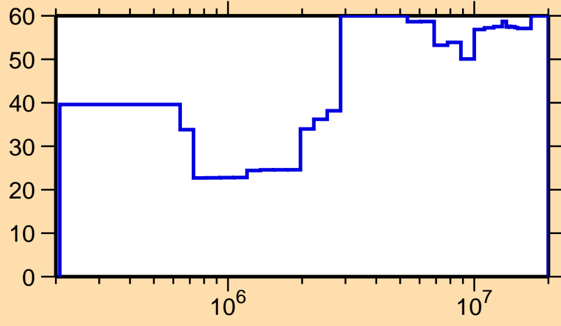
\Delta\sigma/\sigma vs. E for ^{99}\text{Pd}(n,n_1)
