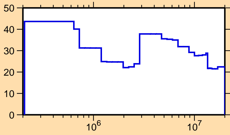
\Delta\sigma/\sigma vs. E for ^{99}\text{Pd}(n,\text{inel.})
