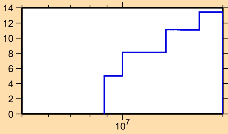
\Delta\sigma/\sigma vs. E for ^{99}\text{Pd}(n,\text{tot.})
