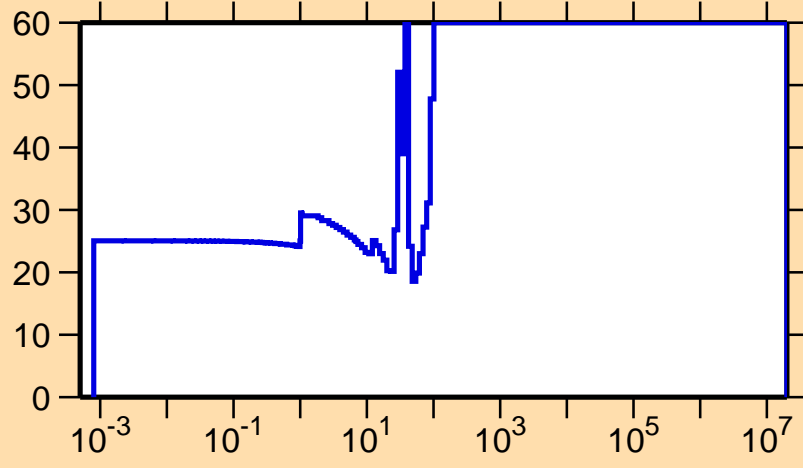
\Delta\sigma/\sigma vs. E for ^{99}\text{Pd}(n,\gamma)
