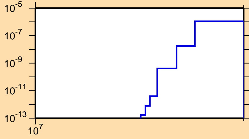
\sigma vs. E for ^{99}\text{Pd}(\text{mt } 45)
