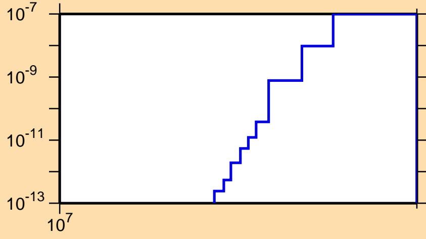
\sigma vs. E for ^{99}\text{Pd}(\text{mt117})
