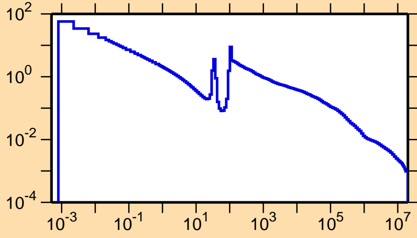
\sigma vs. E for ^{99}\text{Pd}(n,\gamma)
