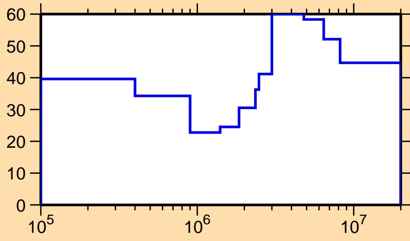
\Delta\sigma/\sigma vs. E for ^{99}\text{Pd}(n,n_1)
