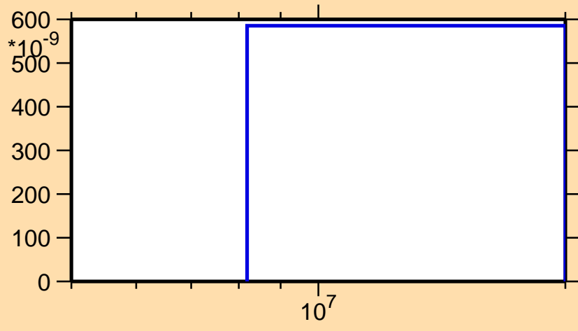
\sigma vs. E for ^{99}\text{Pd}(n,nd)
