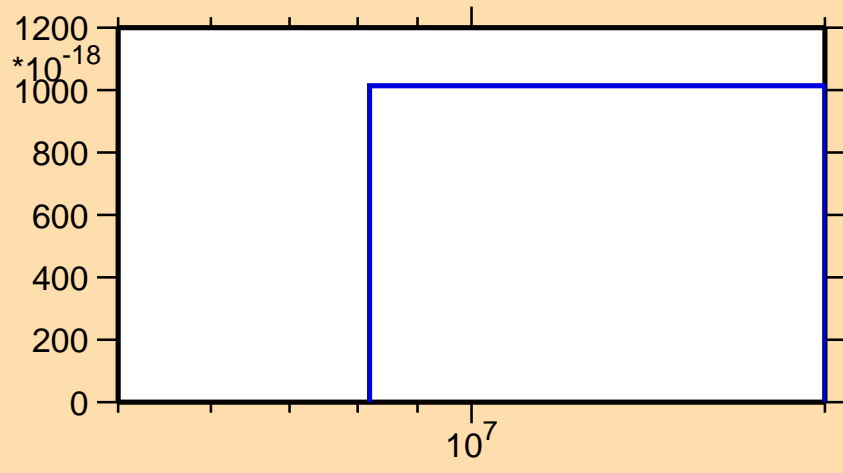
\sigma vs. E for ^{99}\text{Pd}(n,nt)
