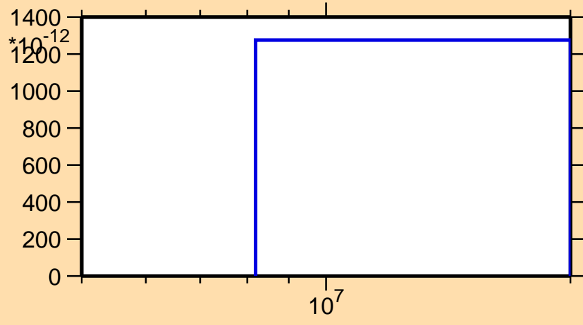
\sigma vs. E for ^{99}\text{Pd}(\text{mt117})
