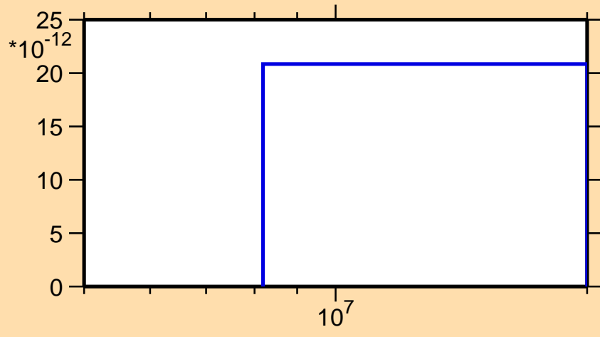
\sigma vs. E for ^{99}\text{Pd}(\text{mt } 34)
