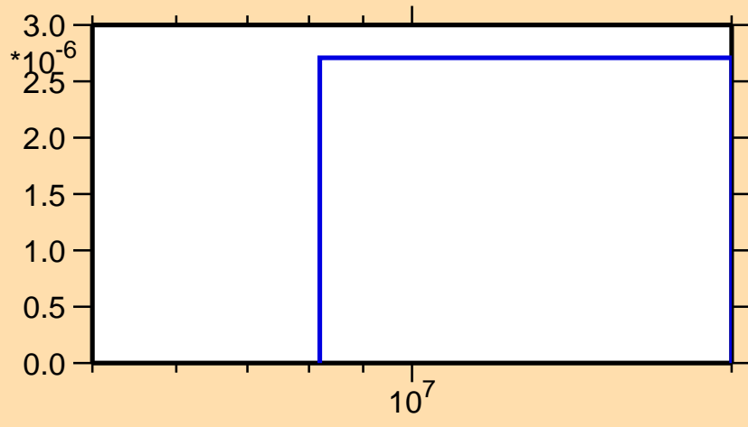
\sigma vs. E for ^{99}\text{Pd}(n,\text{pd})
