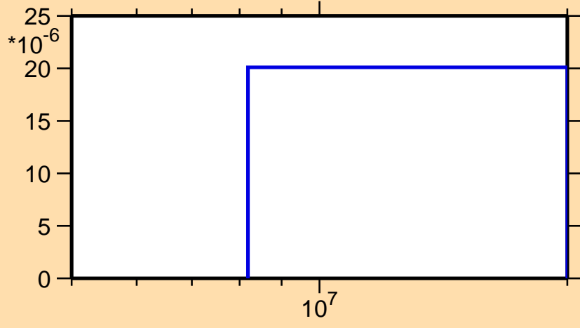
\sigma vs. E for ^{100}\text{Pd}(n,t)
