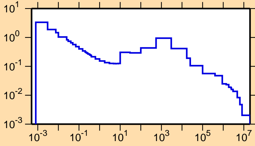
\sigma vs. E for ^{100}\text{Pd}(n,\gamma)
