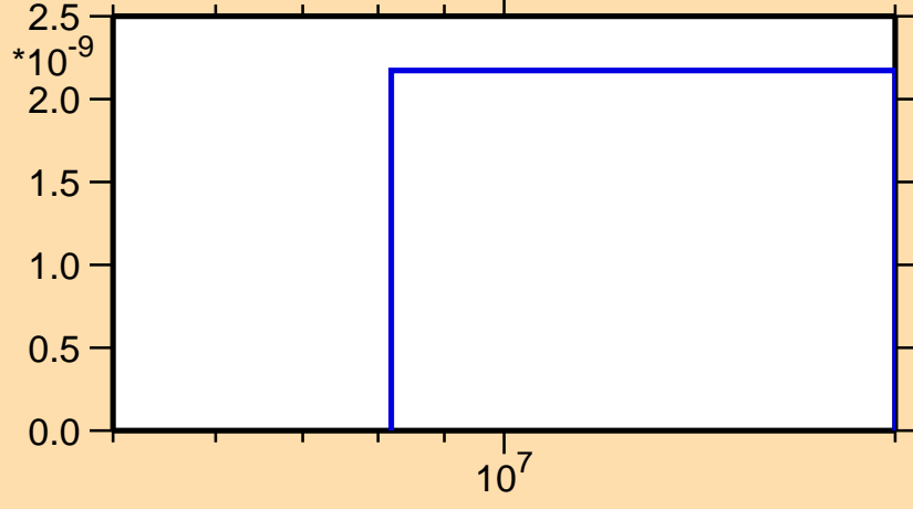
\sigma vs. E for ^{101}\text{Pd}(n,\text{pd})
