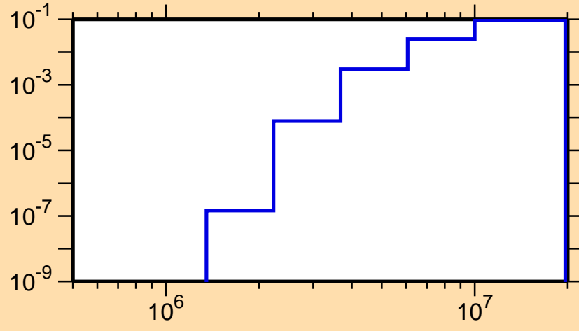
\sigma vs. E for ^{102}\text{Pd}(n,p)
