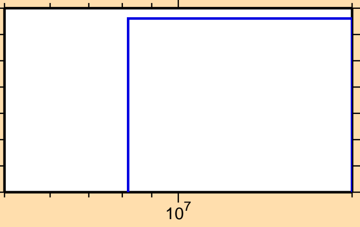
\sigma vs. E for ^{102}\text{Pd}(n,\text{pt})
