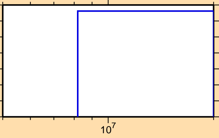
\sigma vs. E for ^{102}\text{Pd}(n,\text{He}3)
