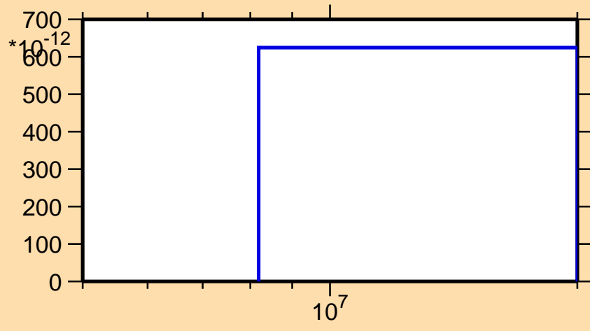
\sigma vs. E for ^{102}\text{Pd}(n,\text{nd})
