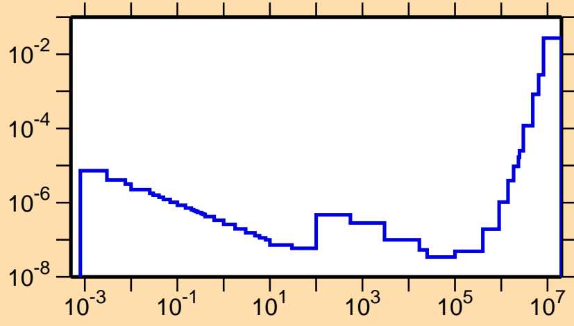
\sigma vs. E for ^{102}\text{Pd}(n,\alpha)
