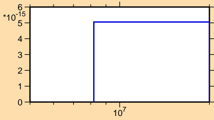
\sigma vs. E for ^{102}\text{Pd}(n,nt)
