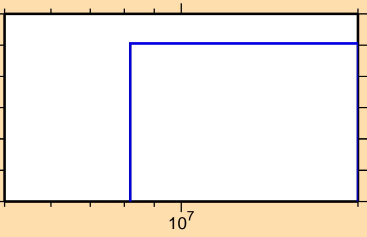
\sigma vs. E for ^{102}\text{Pd}(n,nt)
