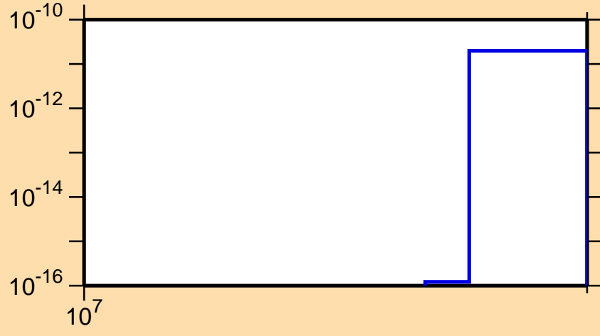
\sigma vs. E for ^{103}\text{Pd}(n,nt)
