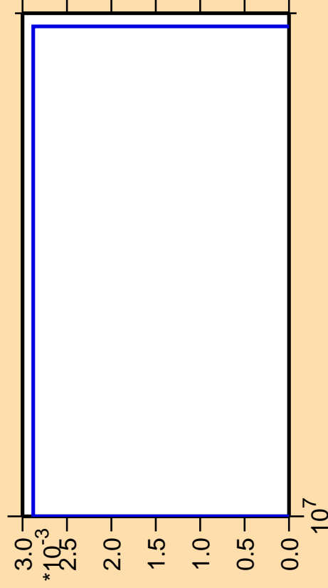
\Delta\sigma/\sigma vs. E for ^{103}\text{Pd}(\text{mt } 45)
