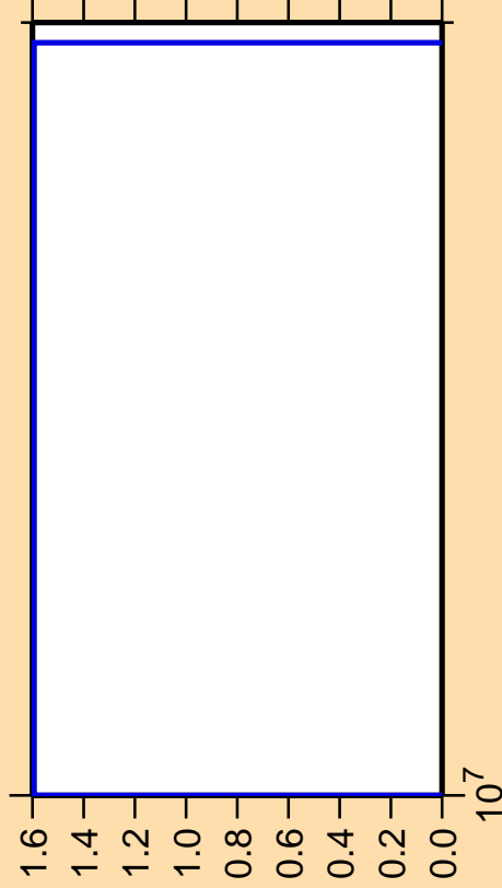
\Delta\sigma/\sigma vs. E for ^{103}\text{Pd}(n,\text{pd})
