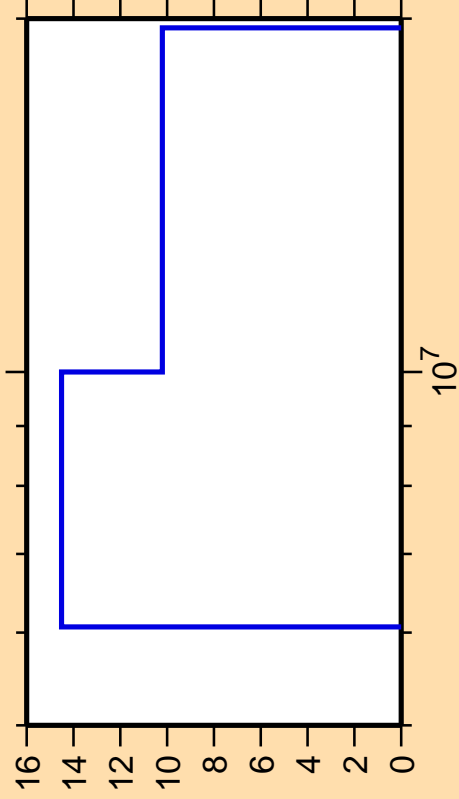
\Delta\sigma/\sigma vs. E for ^{103}\text{Pd}(n,2n)
