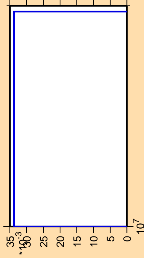
\Delta\sigma/\sigma vs. E for ^{103}\text{Pd} (mt 34)
