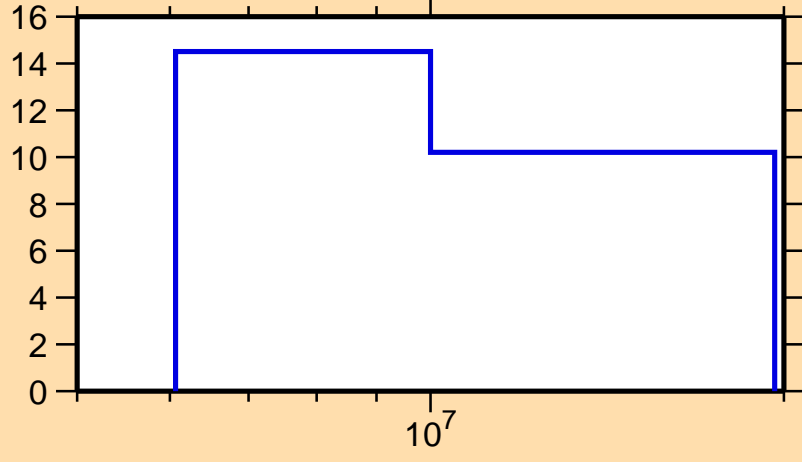
\Delta\sigma/\sigma vs. E for ^{103}\text{Pd}(n,2n)
