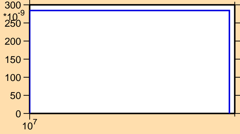
\sigma vs. E for ^{103}\text{Pd}(n,2np)
