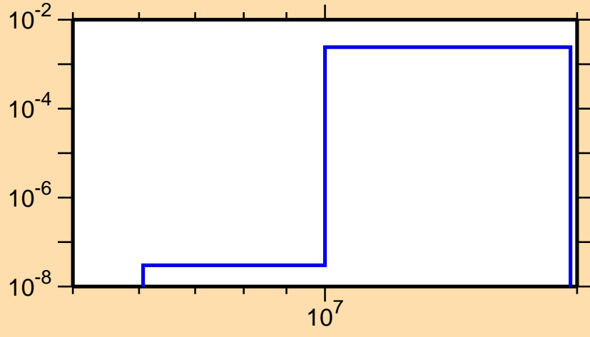
\sigma vs. E for ^{103}\text{Pd}(n,d)
