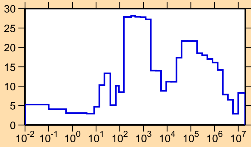
\Delta\sigma/\sigma vs. E for ^{103}\text{Pd}(n,\text{tot.})
