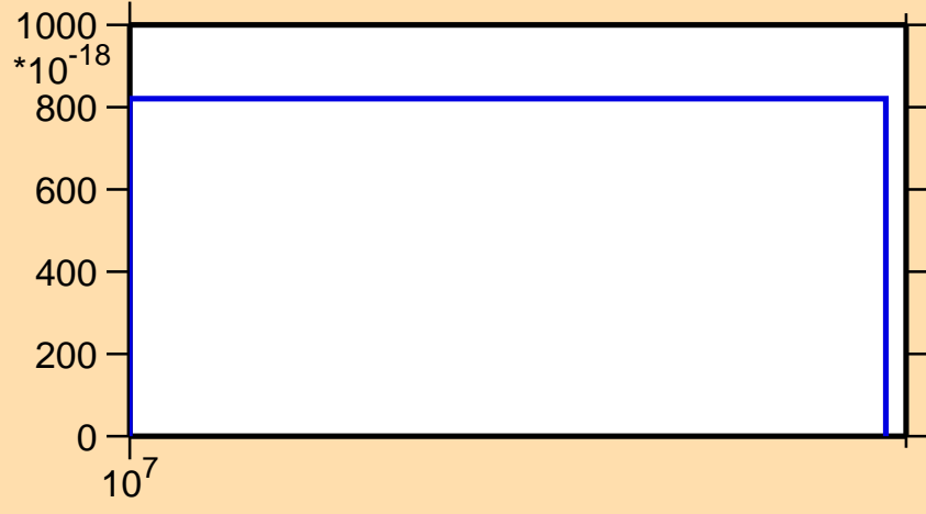
\sigma vs. E for ^{103}\text{Pd}(\text{mt } 45)
