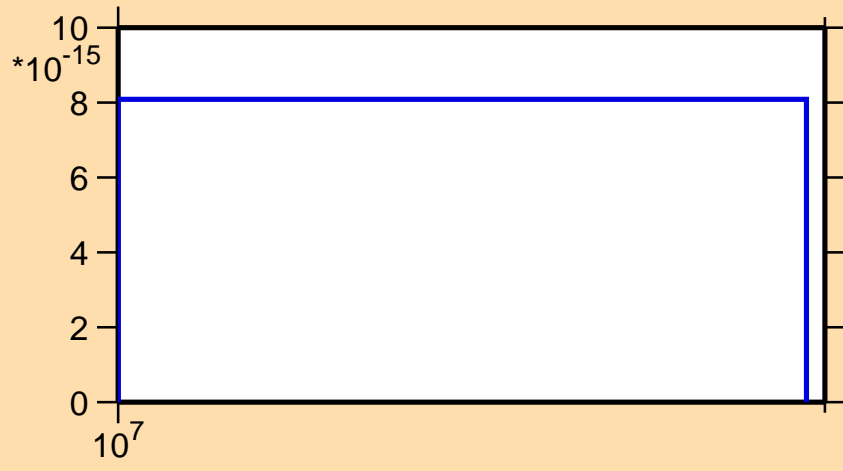
\sigma vs. E for ^{103}\text{Pd} (mt 34)
