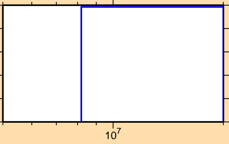
\sigma vs. E for ^{103}\text{Pd}(n,t)
