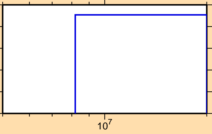
\sigma vs. E for ^{103}\text{Pd}(n,p\alpha)
