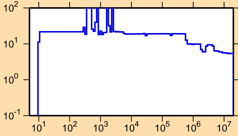
\Delta\sigma/\sigma vs. E for ^{104}\text{Pd}(n,\text{nonel.})
