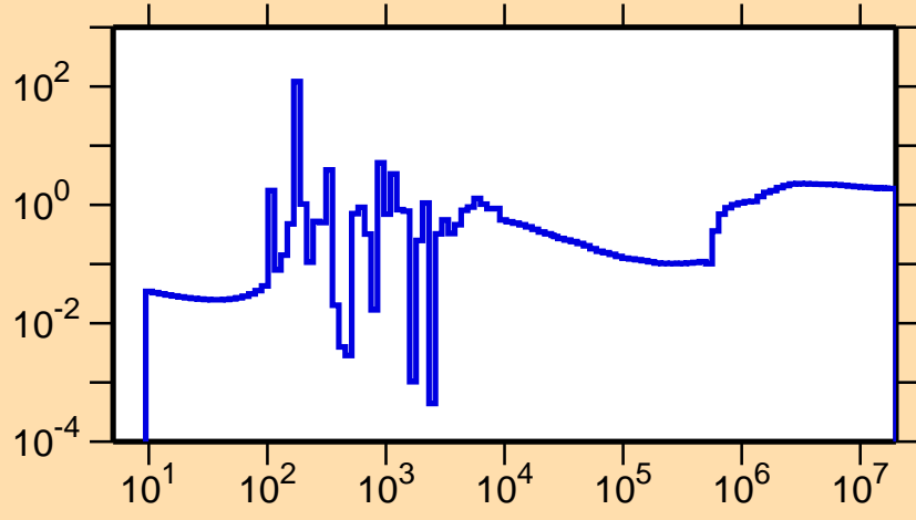
\sigma vs. E for ^{104}\text{Pd}(n,\text{nonel.})
