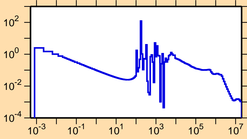
\sigma vs. E for ^{104}\text{Pd}(n,\gamma)
