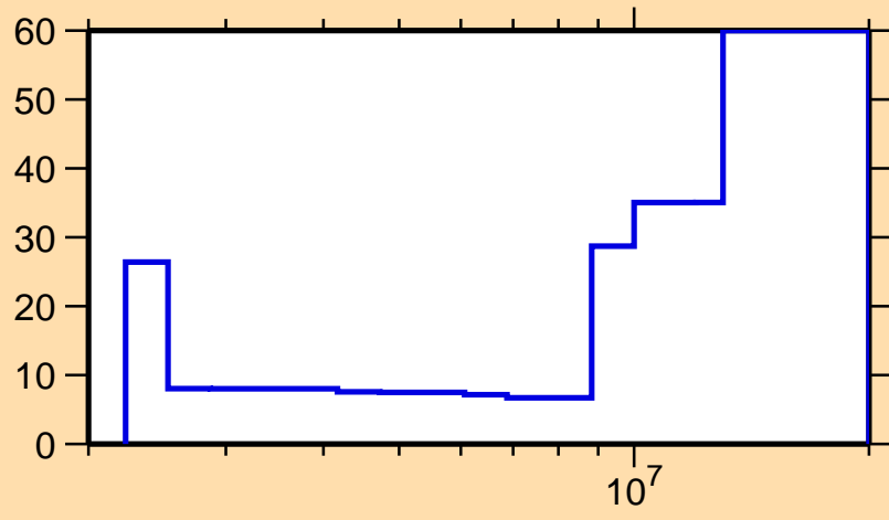
\Delta\sigma/\sigma vs. E for ^{104}\text{Pd}(n,n\text{cont.})
