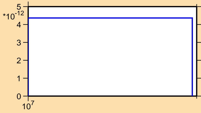
\sigma vs. E for ^{104}\text{Pd}(n,2np)
