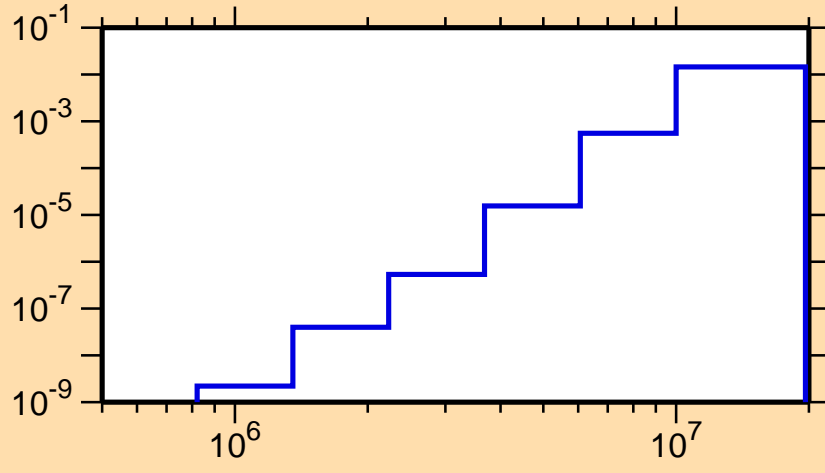
\sigma vs. E for ^{104}\text{Pd}(n,\alpha)
