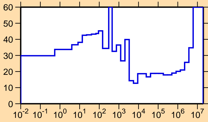
\Delta\sigma/\sigma vs. E for ^{104}\text{Pd}(n,\gamma)
