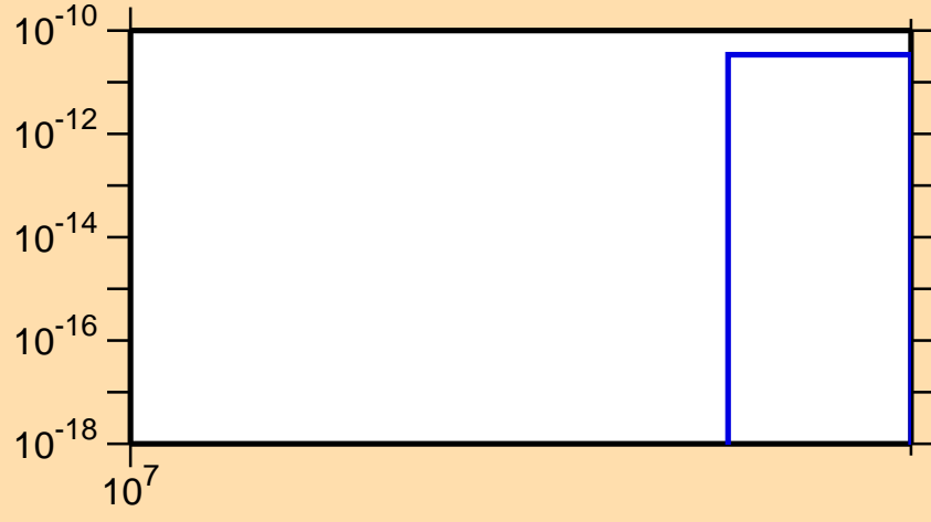
\sigma vs. E for ^{105}\text{Pd}(n,nt)
