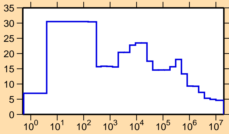
\Delta\sigma/\sigma vs. E for ^{105}\text{Pd}(n,\text{nonel.})
