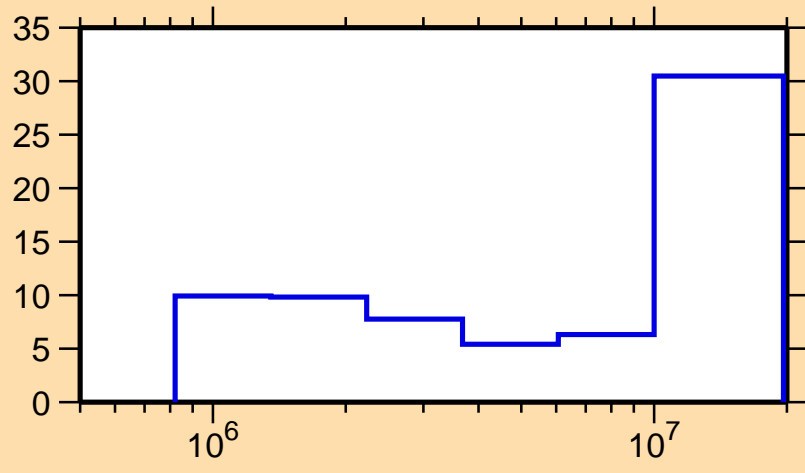
\Delta\sigma/\sigma vs. E for ^{105}\text{Pd}(n,\text{inel.})
