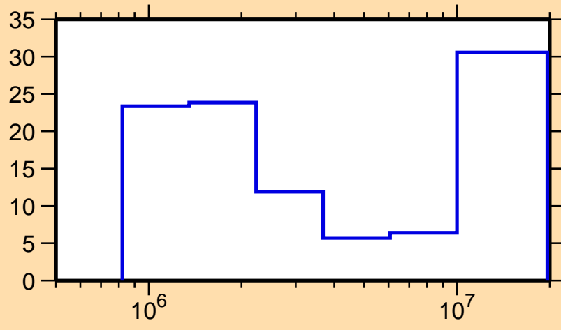
\Delta\sigma/\sigma vs. E for ^{105}\text{Pd}(n,n\text{cont.})
