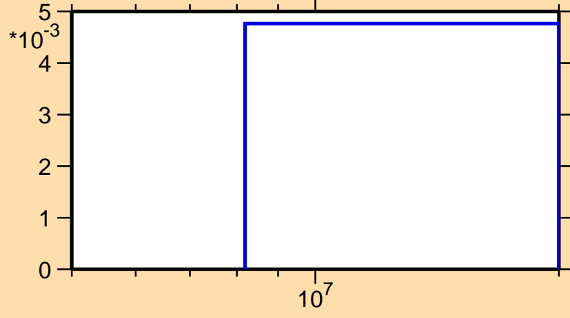
\sigma vs. E for ^{105}\text{Pd}(n,np)
