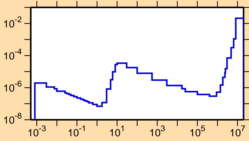
\sigma vs. E for ^{105}\text{Pd}(n,\alpha)
