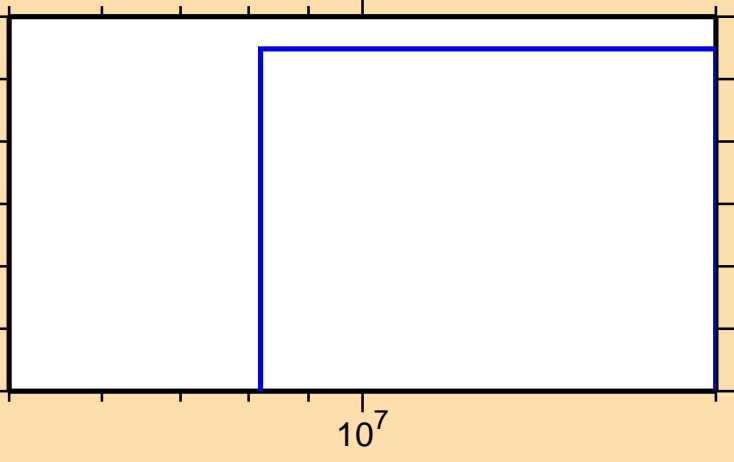
\sigma vs. E for ^{105}\text{Pd}(n,t)
