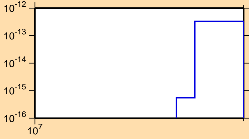
\sigma vs. E for ^{106}\text{Pd}(n,\text{pd})
