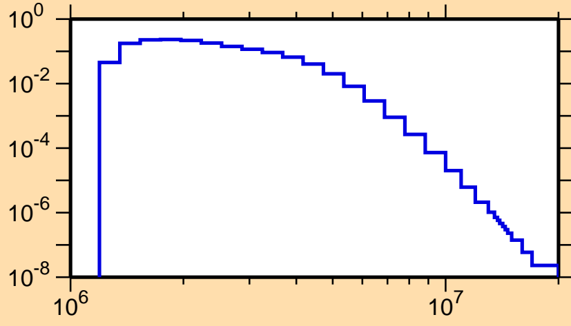
\sigma vs. E for ^{106}\text{Pd}(n,n_4)
