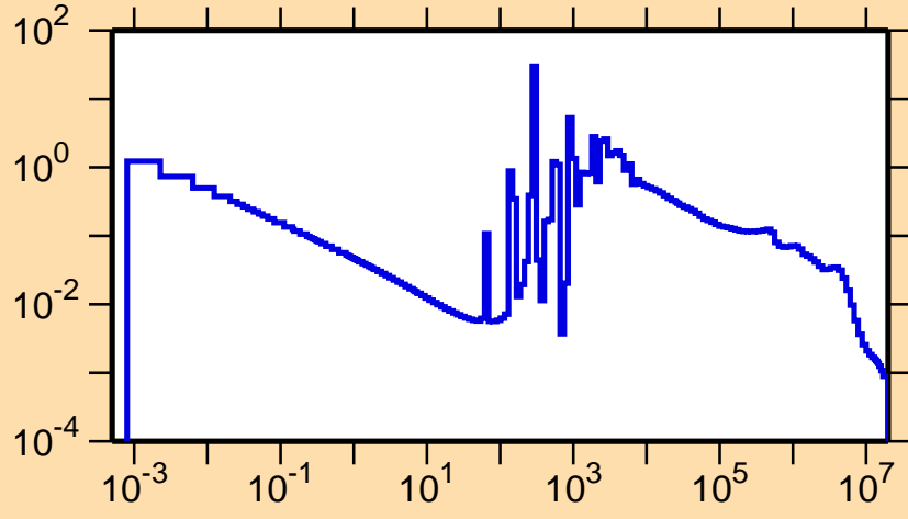
\sigma vs. E for ^{106}\text{Pd}(n,\gamma)
